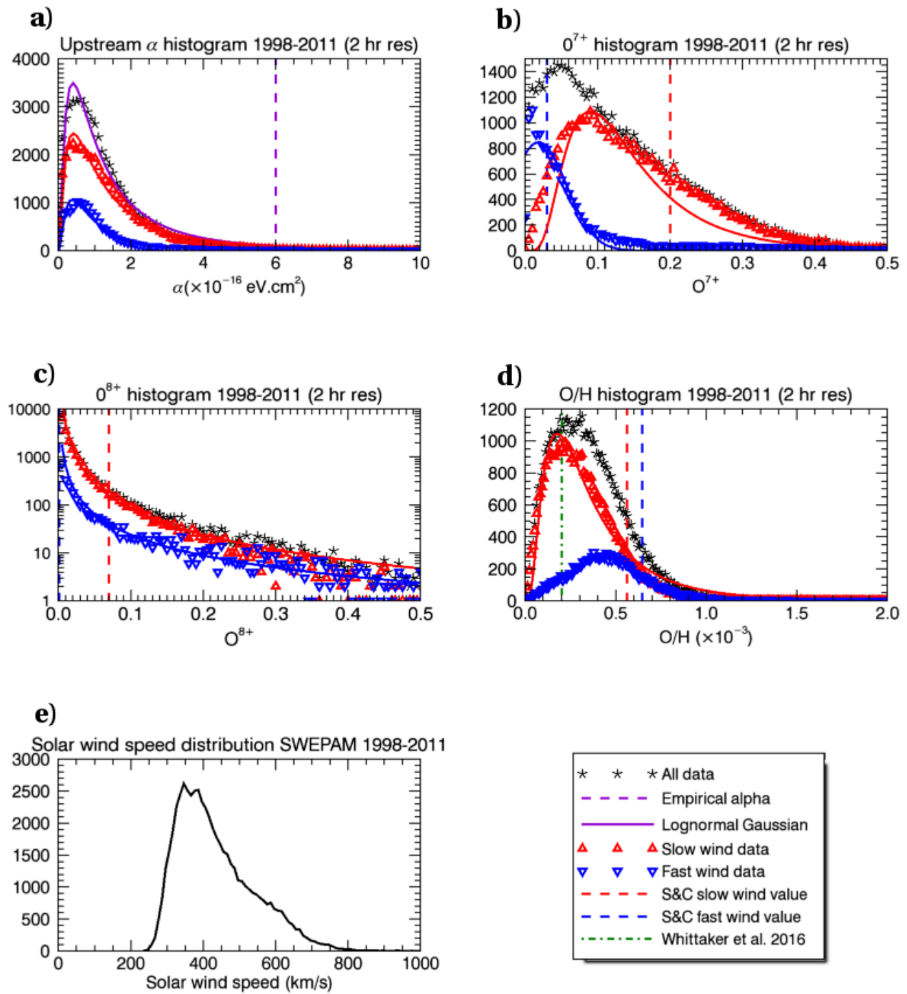
Figure 2. ACE data taken over 13 years showing the fast (blue), slow (red) and all (black) solar wind speed oxygen parameters. a) \alpha_o distributions in the solar wind fitted with lognormal Gaussians. b) O^{7+} distributions with fitted lognormal Gaussians. c) O^{8+} distributions with power law fits. d) O/H distribution in the solar wind. e) The solar wind speed distribution.
