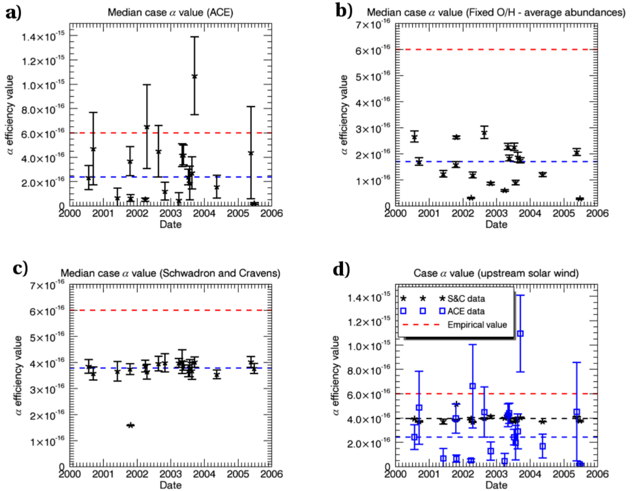
Figure 1. The \alpha_o value for XMM-Newton cases examined in Whittaker et al. [2016] (see Section 3). The all species \alpha empirical value of 6 \times 10^{-16} (red dashed line) and the data averages (blue dashed) are shown. a) the average \alpha_o using ACE abundances. b) the average \alpha_o using the study fixed abundances. c) the average \alpha_o using Schwadron and Cravens [2000] abundances. d) the average \alpha_o in the upstream solar wind comprising, ACE abundances (blue squares) and empirical values (black stars).
