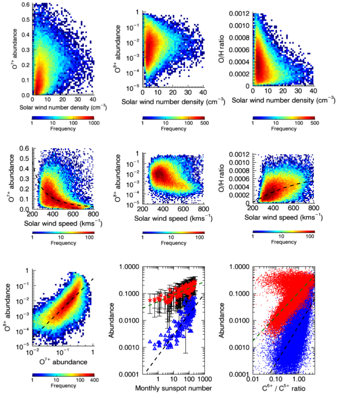
Figure 3. 13 years of ACE oxygen data compared to the solar wind number density (top row), solar wind bulk flow (middle row) and other solar wind parameters (bottom row). a) O^{7+} against n_{sw} , b) O^{8+} against n_{sw} , c) \frac{O}{H} against n_{sw} . d) O^{7+} against v_{sw} , a power law fit is included (black) e) O^{8+} against v_{sw} , f) \frac{O}{H} against v_{sw} , a polynomial fit line is included (black). g) O^{7+} against O^{8+} , a power law fit is shown (black), h) O^{7+} (red) and O^{8+} (blue) scatter points as a function of sunspot number, i) O^{7+} (red) and O^{8+} (blue) scatter points as a function of \frac{C^{6+}}{C^{5+}} .
