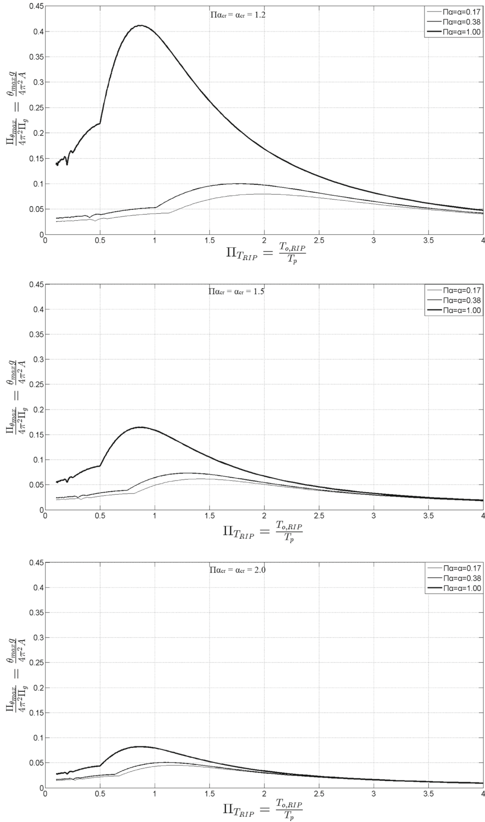
Fig. 7 Dimensionless response spectra of the RIP when subjected to a single sinusoidal pulse with period T_p and amplitude A_p , for different values of \alpha and \alpha_{cr}
