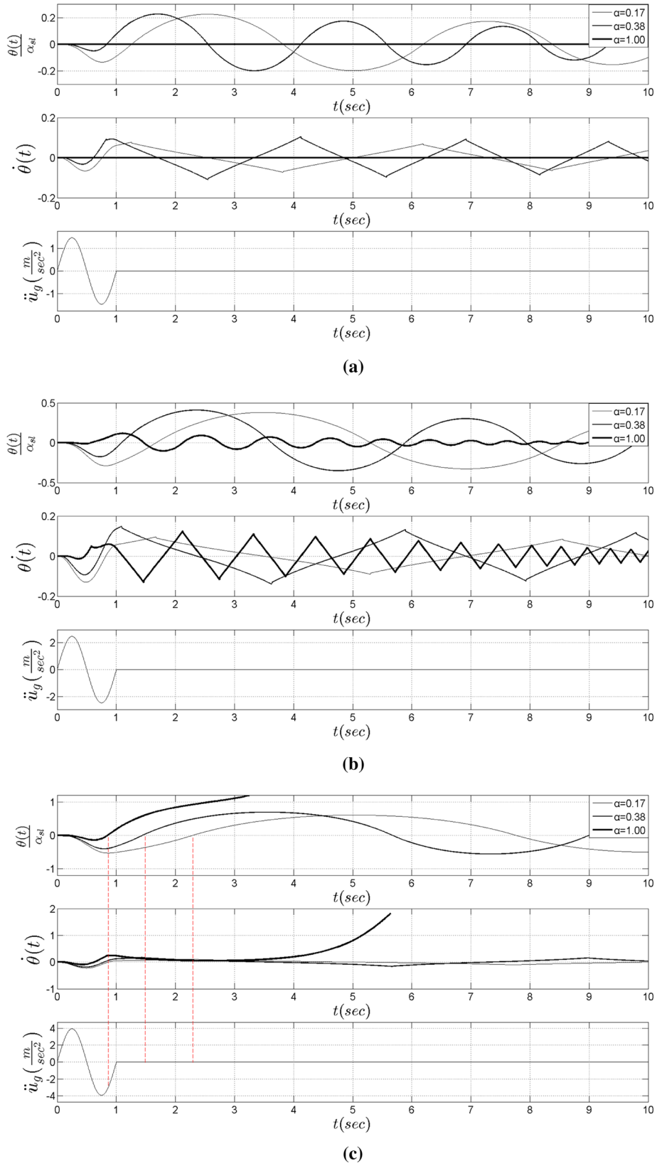
Fig. 13 Rocking response of a RB with R = 7.21 and \alpha_{sl} = 1/4 when subjected to a single sinusoidal pulse with period T_p = 1.00 s, and different amplitudes a A_p = 0.20 g, b A_p = 0.35 g, c A_p = 0.55 g for \alpha = 0.17, 0.38 and 1.00
