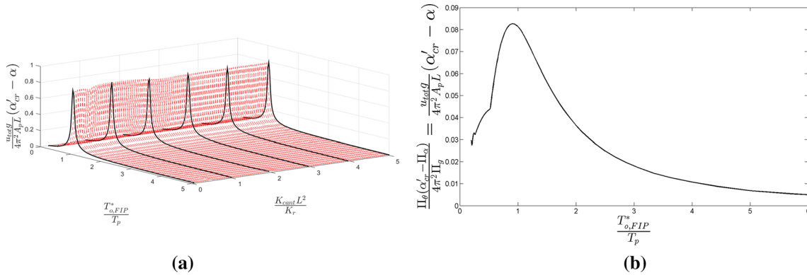
Fig. 10 a 3D Dimensionless self-similar response spectrum of the FIP when subjected to a continuous sine pulse with period T_p and amplitude A_p , b self-similar spectrum curve of a FIP which is subjected to one-cycle sinusoidal pulse with period T_p and amplitude A_p
