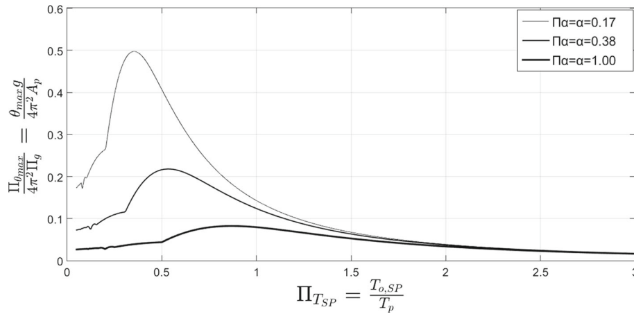
Fig. 3 Dimensionless response spectra of the SP, \frac{\Pi_{\theta_{max}} \Pi_\alpha}{4\pi^2 \Pi_g} , against the dimensionless reference period, \Pi_{T_{SP}} , for the three distinct values of the gravitational multiplier, \Pi_\alpha , when subjected to a single sinusoidal pulse
