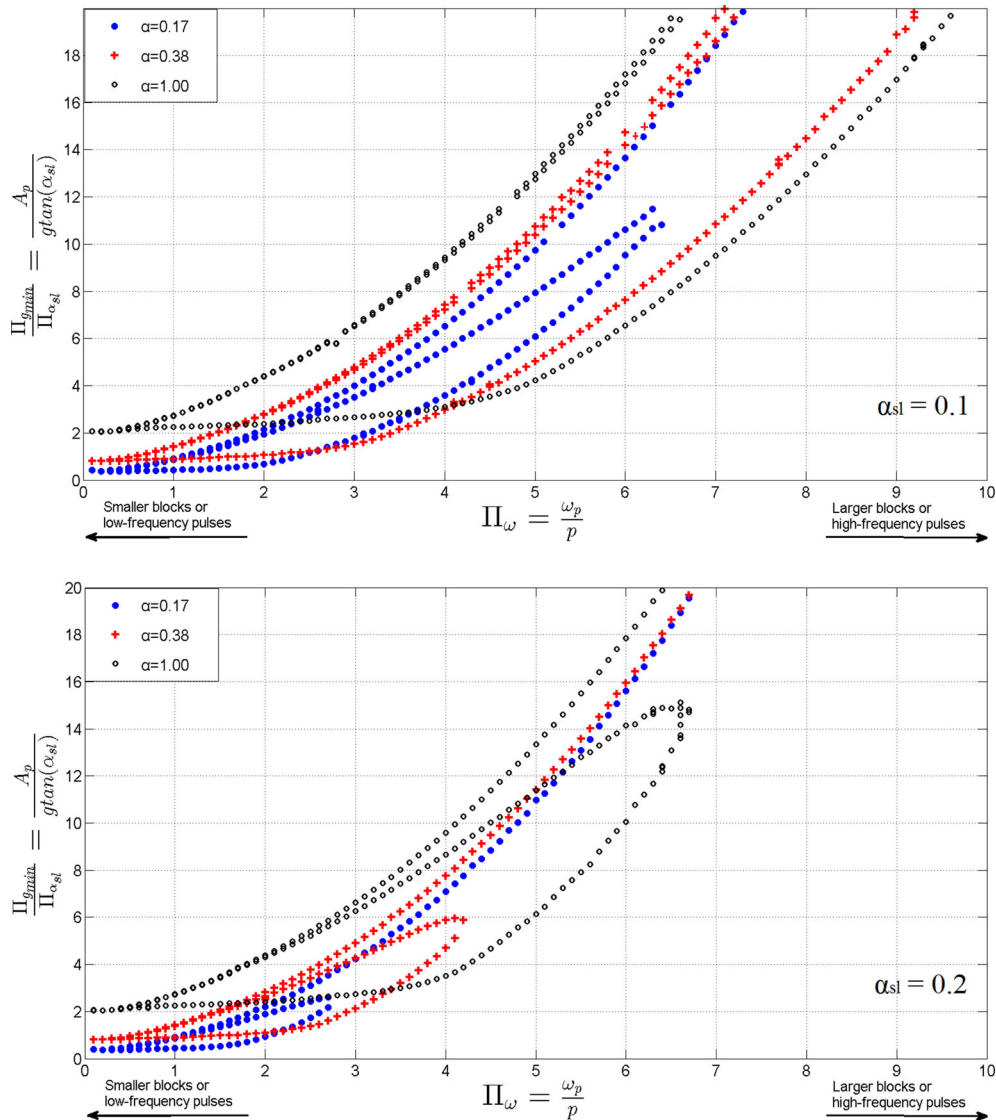
Fig. 20 Rocking spectra of a flexural block when subjected to a sinusoidal pulse for \alpha = \{1.00, 0.38, 0.17\} where: \frac{\omega_n}{p} = 20 , \gamma_{mb} = 1 , \gamma_{mc} = 1
