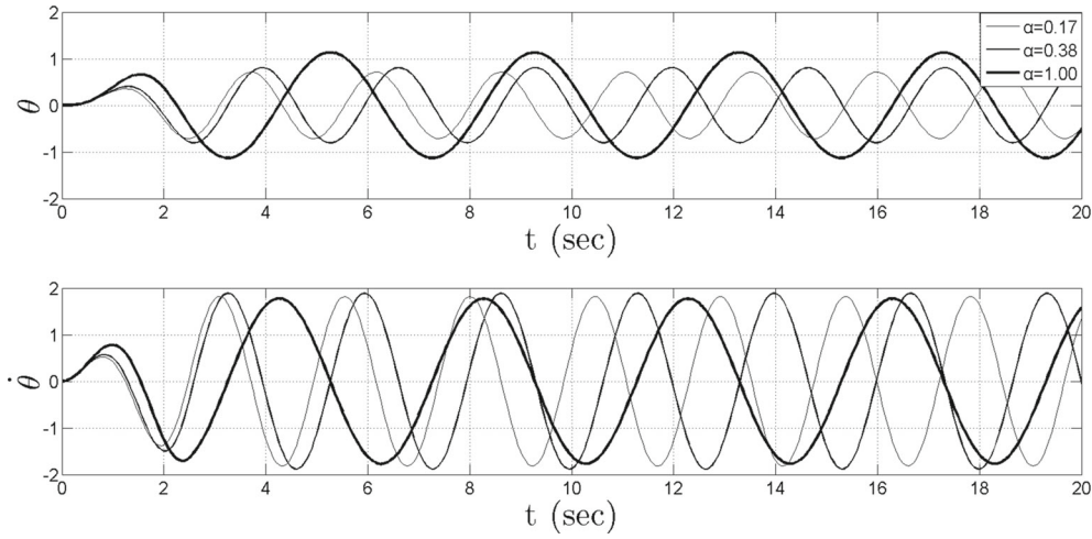
Fig. 5 Time history of a RIP subjected to a single sinusoidal impulse of \Pi_g = 0.3 and T_p = 2.5 s, where T_{0,RIP} = 4.0 s, \Pi_\alpha = \{0.17, 0.38, 1.00\} and \Pi_{\alpha_{cr}} = 1.5
