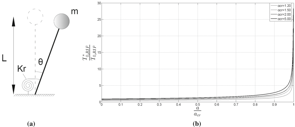
Fig. 4 a Rigid inverted pendulum (RIP); b the influence of the gravitational multiplier \alpha on the natural period of the system
