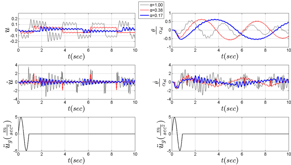
Fig. 17 Rocking response of a flexural block when subjected to a sinusoidal pulse for \alpha = \{1.00, 0.38, 0.17\} where: \frac{\omega_n}{p} = 5, \gamma_{mb} = 2, \gamma_{mc} = 1, \frac{\omega_p}{p} = 7, \frac{A_p}{g \tan(\alpha_{sl})} = 5, \alpha_{sl} = 0.1
