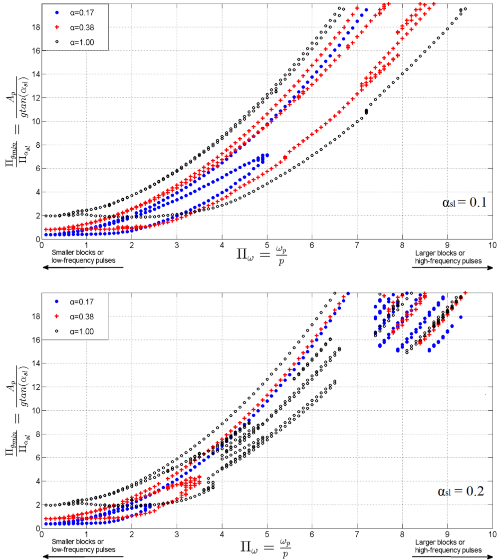
Fig. 19 Rocking spectra of a flexural block when subjected to a sinusoidal pulse for \alpha = \{1.00, 0.38, 0.17\} where: \frac{\omega_n}{p} = 5 , \gamma_{mb} = 1 , \gamma_{mc} = 1
