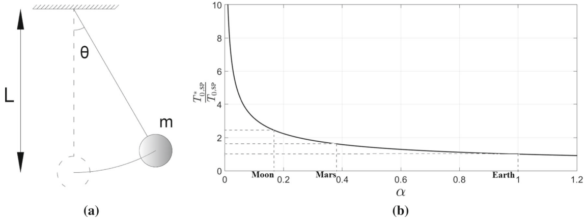
Fig. 1 a Simple harmonic pendulum; b the influence of the gravitational acceleration \alpha to the natural period of the system by assuming zero damping
