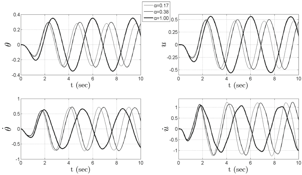
Fig. 9 Time history of a FIP subjected to a sinusoidal impulse of \Pi_g = 0.3 and T_p = 2 s, where T_{0,SP} = 3.47 s, \Pi_\alpha = \{0.17, 0.38, 1.00\} , \Pi_{\alpha_{cr}} = 3.0 and \Pi_k = 2.0
