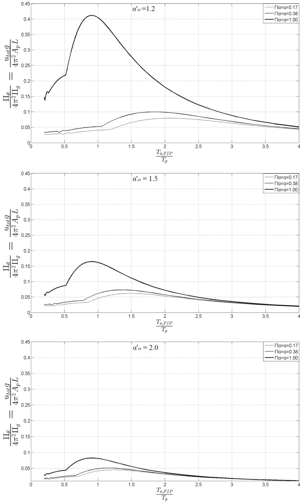
Fig. 11 Dimensionless response spectra of the flexural inverted pendulum FIP when subjected to a sine pulse with period T_p and amplitude A_p , for different values of \alpha and \alpha'_{cr}
