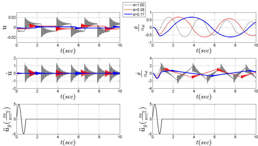
Fig. 18 Rocking response of a flexural block when subjected to a sinusoidal pulse for \alpha = \{1.00, 0.38, 0.17\} where: \frac{\omega_n}{p} = 20, \gamma_{mb} = 2, \gamma_{mc} = 1, \frac{\omega_p}{p} = 7, \frac{A_p}{g \tan(\alpha_{sl})} = 5, \alpha_{sl} = 0.1
