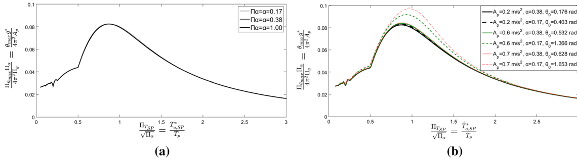
Fig. 2 a Dimensionless response spectrum of an SP subjected to a one-cycle sinusoidal pulse, exhibiting self-similar behavior for a large range of dimensionless periods, T_{0,SP}^*/T_p , obtained by considering a small-angle approximation; b the influence of the angular response in the dimensionless response spectrum of an SP, subjected to a one-cycle sinusoidal pulse
