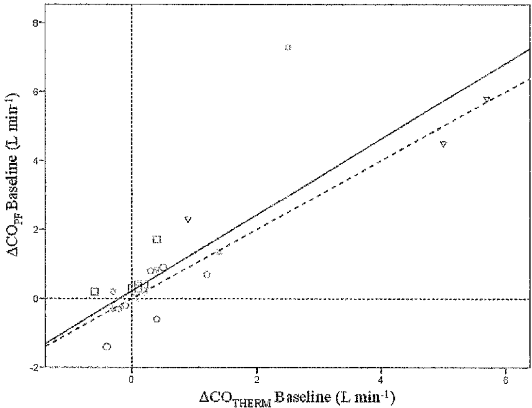
Figure 3.5a: Comparison change of physioflow derived cardiac output from baseline, \Delta CO_{PF} \text{ Baseline (L min}^{-1}\text{)} , during all the physiological situations compared with that of the change from baseline of thermodilutional derived cardiac output, \Delta CO_{THERM} \text{ Baseline (L min}^{-1}\text{)} , in the 21 individuals ( n=26 ). The individual diseases with the paired data of normal subjects shown by an inverse purple triangle, idiopathic pulmonary arterial hypertension (IPAH) by a red hexagon, Connective tissue disorders (CTD) by a green square, Chronic obstructive pulmonary disease (COPD) by a dark blue circle, interstitial lung disease shown with a tanned upright triangle and Chronic thromboembolic pulmonary hypertension by a light blue star. The line of identity given by the broken black line, and the regression line for the combined paired data sets, by the continuous black line.
