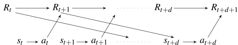
Fig. 4.1 Section of the perception–action loop represented as a Bayesian network with fixed time delay ( d ) between actuation ( a ) and sensing ( s ), closed through the environment ( R ).
