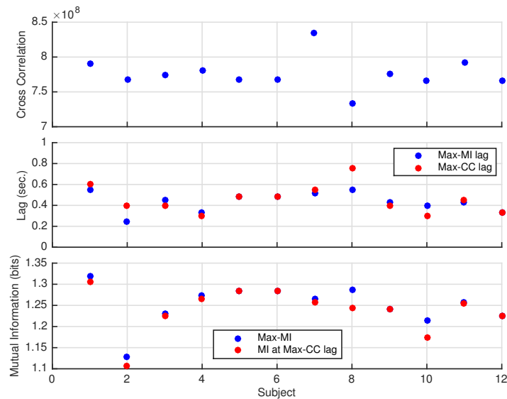
Fig. 5.8 Cross Correlation (top) and Mutual Information (bottom) of perception and action in the condition ‘High’ of Experiment I. High levels of cross correlation with low variability (top). The lags between perception and action maximising cross correlation (red) and mutual information (blue) reflect the human sensorimotor delay of 300-500 ms (middle). The levels of mutual information between perception and action maximised over lags (blue) and computed for maximal cross correlation lags (red) are upper-bounded by 1.58 bits (bottom).
