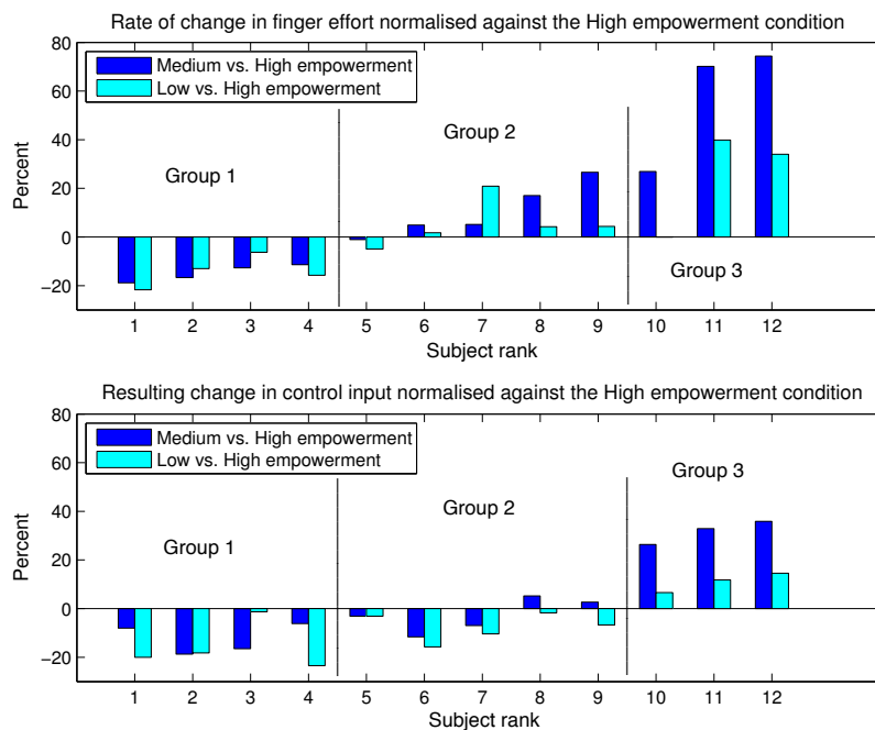
Fig. 4.7 Change in finger movement effort (top) and the resulting change in control input (bottom) – subjects are ranked according to performance in the Medium vs. High empowerment condition in the top and the same ranking is used in the bottom. The Medium and Low empowerment conditions are normalised against the High.
