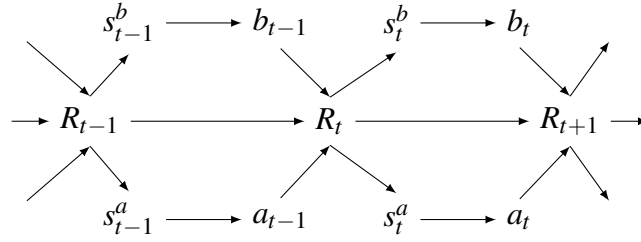
Fig. 8.2 Section of the causal Bayesian network representing the perception–action loop of a dyad ( A - B ) interacting through the environment ( R ) by applying actions ( a and b ) in response to sensor stimuli ( s^a and s^b ) unrolled over time.
