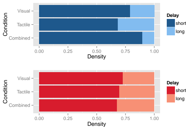
Fig. 8.7 Cumulative delay density profile for all three experimental conditions. Short delays refer to the [-2.5,2.5] seconds interval and long delays to larger levels. Category 1 (top) reveals higher density of short delays in the Combined than in the Visual condition, whereas Category 2 (bottom) shows lower levels and little variation across conditions.
