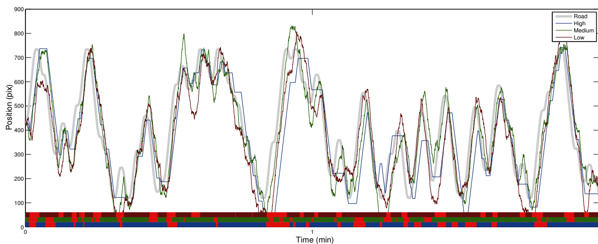
Fig. 4.9 Time series of subject B, an example of low expended effort, in the High (blue), Medium (green) and Low (brown) empowerment conditions. Lag patterns of relaxed target-following are visible at the peaks. The colour strips underneath depict events on/off-target. The red blocks reveal a significant number of periods off-target of considerable length.
