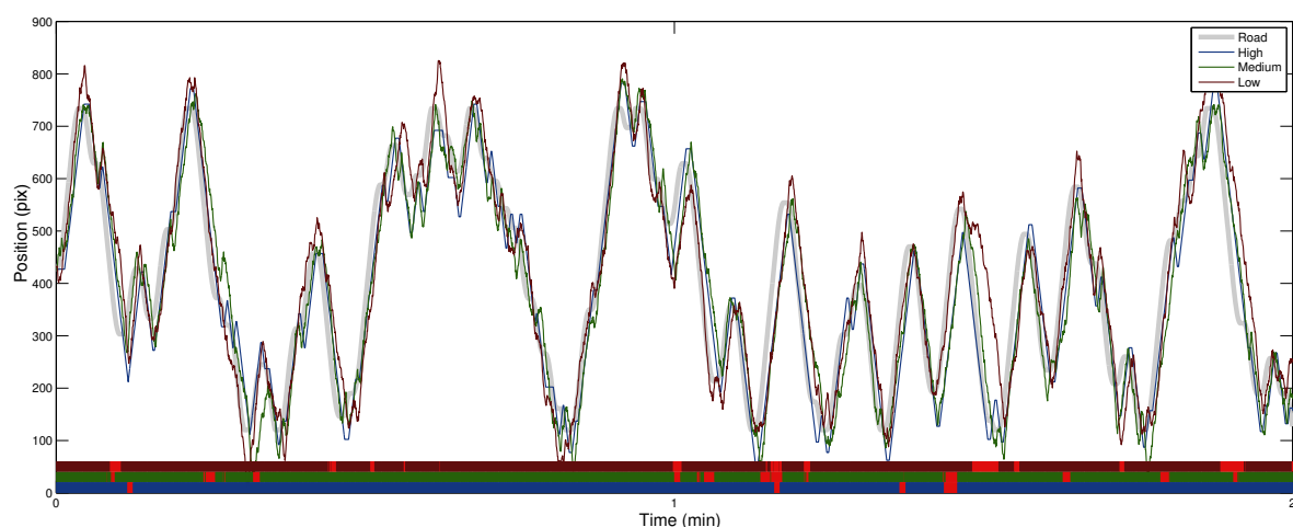
Fig. 4.8 The time series of subject A in the High (blue), Medium (green) and Low (brown) empowerment conditions – an example of high expended effort. Lead patterns of target-anticipating behaviour are visible at the turning points. The colour strips underneath represent the events on/off-target. The red blocks show few periods off-target, more frequent in the Medium and the Low empowerment conditions as well as the second half of the sessions.
