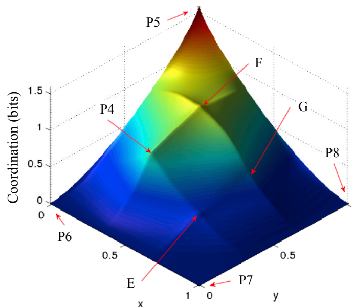
Fig. 8.13 The coordination levels computed on simulated PDFs generated with a linear interpolation on the three empirical (F, G, E) and five artificial (P4-P8) densities. P5 corresponds to tightly-coupled controllers yielding the theoretical maximum for this model of \log 3 = 1.58 bits. P6 – P8 correspond to different types of non-coordinated behaviour.
