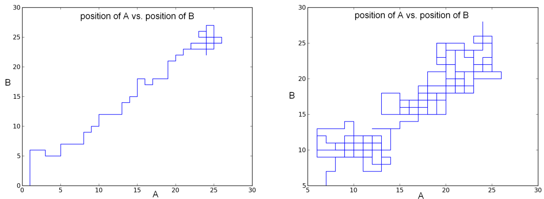
Fig. 7.8 Simulated trajectories of agent A vs. agent B for r_t = 1 range of contact and (a) delay = 0, \sigma^2 = 0 , (b) delay = 4, \sigma^2 = 2 reflecting patterns of a tight (left) and a chaotic (right) tracking behaviour.
