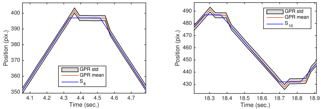
Fig. 5.17 Regression mean (red) and standard deviation (grey) of SSGP models for subjects S_8 (left) and S_{10} (right) derived with 100 basis functions, revealing a close fit with a minor overshoot around the turning points.
