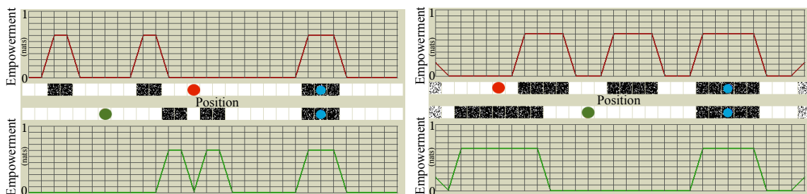
Fig. 7.3 Visualisation of 1-step (left) and 2-step (right) empowerment in the case of deterministic state transitions ( \sigma_0^2 = 0, \sigma_1^2 = 0 ) using two ranges of contact – r_t^A = 3 for agent A and r_t^B = 1 for agent B. The empowerment levels are represented by green and red curves as well as by density clouds. Inside larger contact regions empowerment is zero (top). 2-step action sequences inflict the merger of the two basins of high empowerment (bottom/right).
