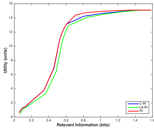
Fig. 5.5 The empirical trade-off curves computed on simulated data obtained from executing the optimal RI, C-RI and LA-RI policies corresponding to various levels of \beta . The deviations from the theoretical curves are due to the fixed initial starting state used in all simulations, which restricts the number of visited states.
