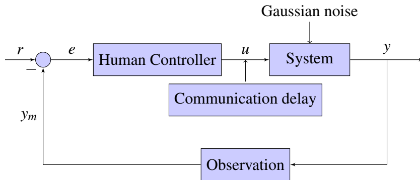
Fig. 4.2 Human as an operator – a control system view of the HCI feedback loop.
