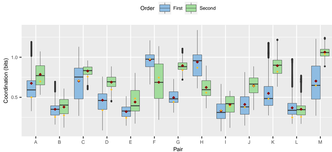
Fig. 8.19 Within-pair variability of the coordination levels in the Visual and the Combined conditions in their respective trial order computed on 60-seconds wide sliding windows – mean (red dots). Overall coordination levels are computed on the full data sets (yellow dots). A marked learning effect is visible for pairs C, D, G, K and M.
