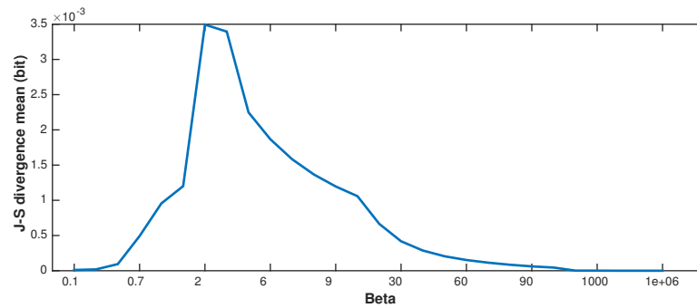
Fig. 5.2 The Jensen-Shannon divergence mean between the optimal LA-RI and C-RI policies computed for various levels of \beta . The policies are most distinct for \beta = 2 and coincide at the two extremes.
