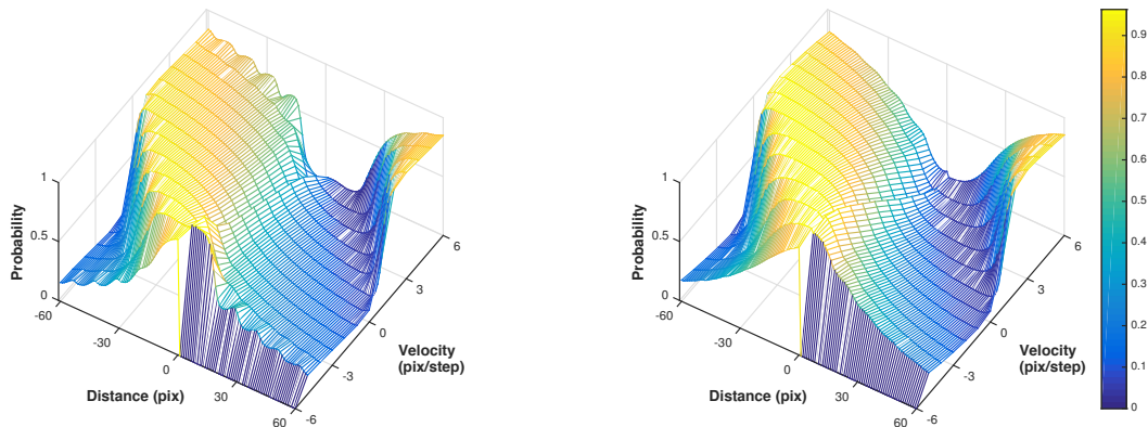
Fig. 5.4 The optimal C-RI (left) and LA-RI (right) policies of a moving action derived for \beta = 2 . The probabilistic profile of the opposite action is symmetrical with an identical shape. For higher velocities LA-RI provides smooth policy transitions unlike C-RI.
