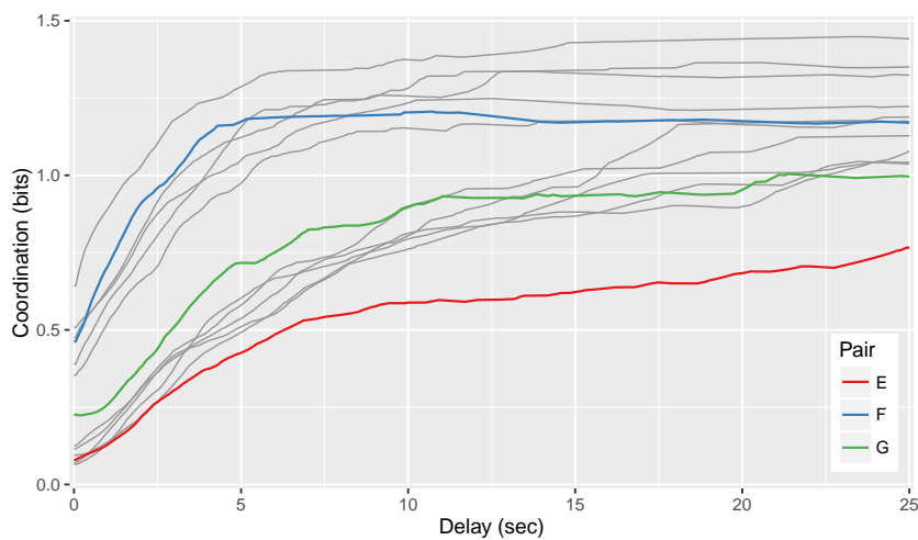
Fig. 8.10 Trade-off curves of the coordination level vs. delay compensation computed for all pairs in the Combined condition. The coordination levels and the saturation rate split the pairs into two distinct groups formed around the blue and the green curves. Larger delays introduce higher variability and a single outlier depicted in red.
