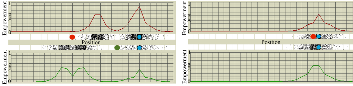
Fig. 7.5 Visualisation of 1-step empowerment in the case of stochastic state transitions ( \sigma_0^2 = 0.7, \sigma_1^2 = 1.5 ) using various ranges of contact – r_t^A = 1, r_t^B = 3 (left) and r_t^A = 0, r_t^B = 0 (right). The empowerment levels are represented by green and red curves as well as by density clouds. The two basins of high empowerment merge at the target providing the highest peak (top/left). The ranges of contact are reduced to zero at the target for both A and B resulting in a single peak (right).
