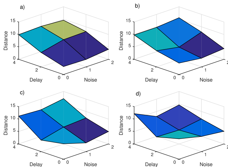
Fig. 7.6 Average number of steps until successful target acquisition per twenty simulated trials in each condition for four levels of the contact range: (a) r_t = 1 , (b) r_t = 2 , (c) r_t = 3 , (d) r_t = 4 . Performance drops with increased uncertainty, however incrementing the contact range introduces a damping effect on disturbances and improving efficiency.
