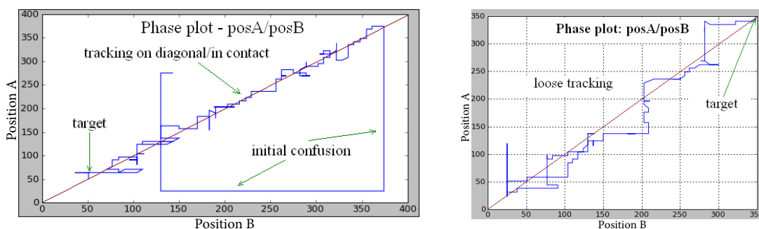
Fig. 7.11 Examples of tight (left) and loose (right) tracking performance provided by the experimental trajectories of subjects A and B in the Combined condition of Experiment II.
