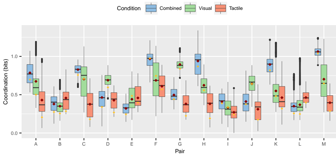
Fig. 8.16 Within-pair variability of the coordination levels for all pairs in the three experimental conditions computed on 60-seconds wide sliding windows – mean (red dots), and the overall coordination levels computed on the full data sets (yellow dots). A high level of coordination with a low variability reveals a consistently good performance.
