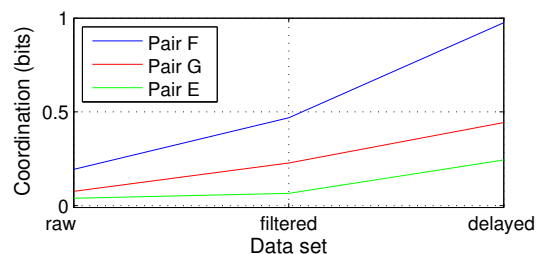
Fig. 8.11 Overall levels of coordination computed for pairs F, G and E (see Figure 8.3) from – (a) raw data, (b) noise-filtered data, and (c) delay-compensated noise-filtered data.
