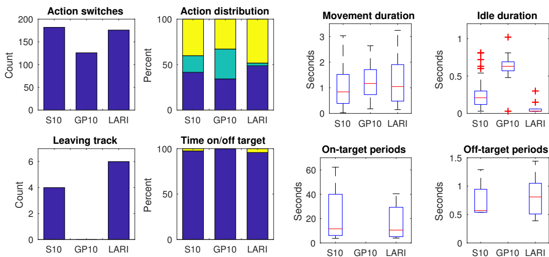
Fig. 5.20 Performance indicators for subject S_{10} , the corresponding Gaussian Process regression model GP_{10} and a LA-RI information-parsimonious model operating with 300 ms actuation delay. S_{10} and LA-RI show similar levels for all indicators, but action distribution and idle periods duration, while GP_{10} achieves the best performance with the least effort.
