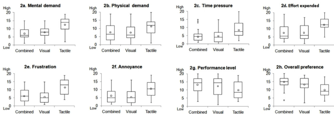
Fig. 1 Results of the extended NASA-TLX questionnaire measuring perceived workload on a 20-point scale. Lower scores correspond to better ratings except for Perceived Performance and Overall Preference, which are reversed. Tactile is generally inferior to the other two conditions.
