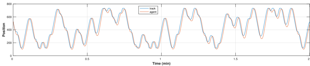
Fig. 5.18 Tracking trajectory of the SSGP model of subject S_{10} , derived with 100 basis functions, generated in simulation with previously unseen track in predictive mode, revealing short lags, smooth transitions and minor overshoot around the turning points.
