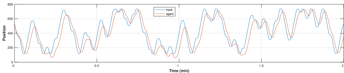
Fig. 5.19 Tracking trajectory of the SSGP model of subject S_8 , derived with 100 basis functions, generated in simulation with previously unseen track in predictive mode, characterised by larger lags and smooth transitions.
