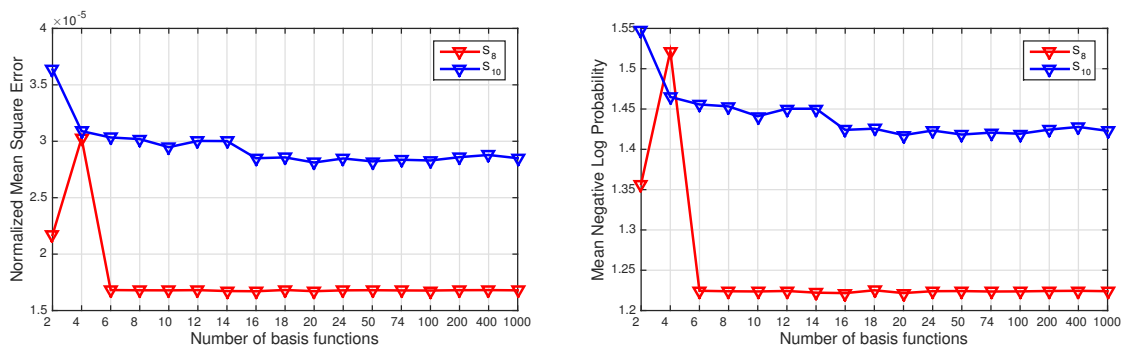
Fig. 5.16 Normalised mean square error (left) and mean negative log-probability (right) of SSGP models trained on experimental data of subjects S_8 (red) and S_{10} (blue) for various numbers of basis functions. The model accuracy is significantly higher for S_8 than for S_{10} , and furthermore saturates the indicators for six vs. 20 basis functions respectively.
