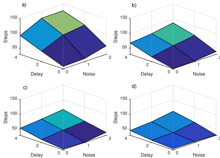
Fig. 7.6 Average number of steps until successful target acquisition per twenty simulated trials in each condition for four levels of the contact range: (a) r_t = 1 , (b) r_t = 2 , (c) r_t = 3 , (d) r_t = 4 . Performance drops with increased uncertainty, however incrementing the contact range introduces a damping effect on disturbances and improving efficiency.
