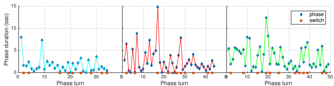
Fig. 6.17 The duration of consecutive phases (blue diamonds) and changes in turn-taking leadership (red squares) in the Visual (left), the Spatial Audio-tactile (middle) and the Audio-tactile (right) condition of a pair performing relatively well in the eyes-free environments. Performance is characterised by intensified interaction and reducing phases.
