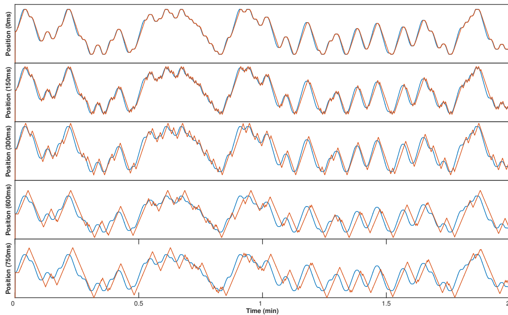
Fig. 5.15 Tracking trajectories of a LA-RI optimal controller ( \beta = 10^6 ) with actuation delay of various magnitudes: 0, 150, 300, 600 and 750 ms (from the top down). Increasing delays introduce lags, overshoot and oscillations around turning points.
