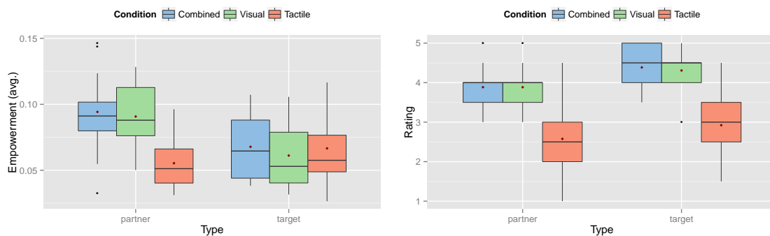
Fig. 7.12 Evaluation of data recorded in Experiment II presenting (a) the average empowerment, which reflects the relative time spent by both subjects in places of high empowerment at the edge of the partner's contact zone (left) or at the target (right) and (b) the subjective ratings indicating how easy it is to locate the partner (left) and the target (right).
