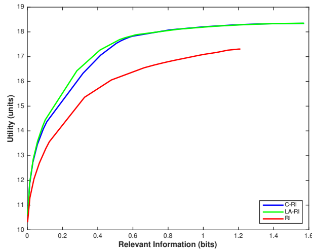
Fig. 5.1 The theoretical information vs. utility trade-off curves generated by the look-ahead (LA-RI), the consistent (C-RI) and the standard (RI) relevant information methods in green, blue and red respectively. RI has lower utility due to the uniform state distribution. LA-RI achieves higher utility than C-RI for a range of finite \beta levels.
