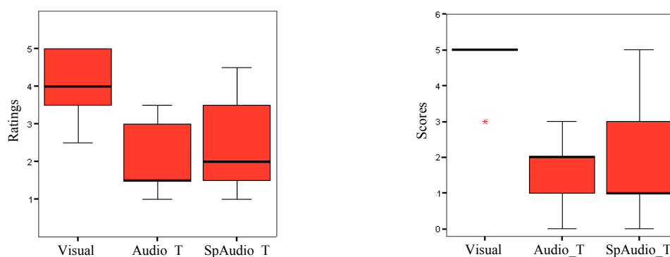
Fig. 6.14 The perceived (left) and the measured performance – number of targets acquired (right) in all three conditions. The perceived performance in the Spatial Audio-tactile is significantly higher than the Audio-tactile condition ( p = .036 with Bonferroni correction).
