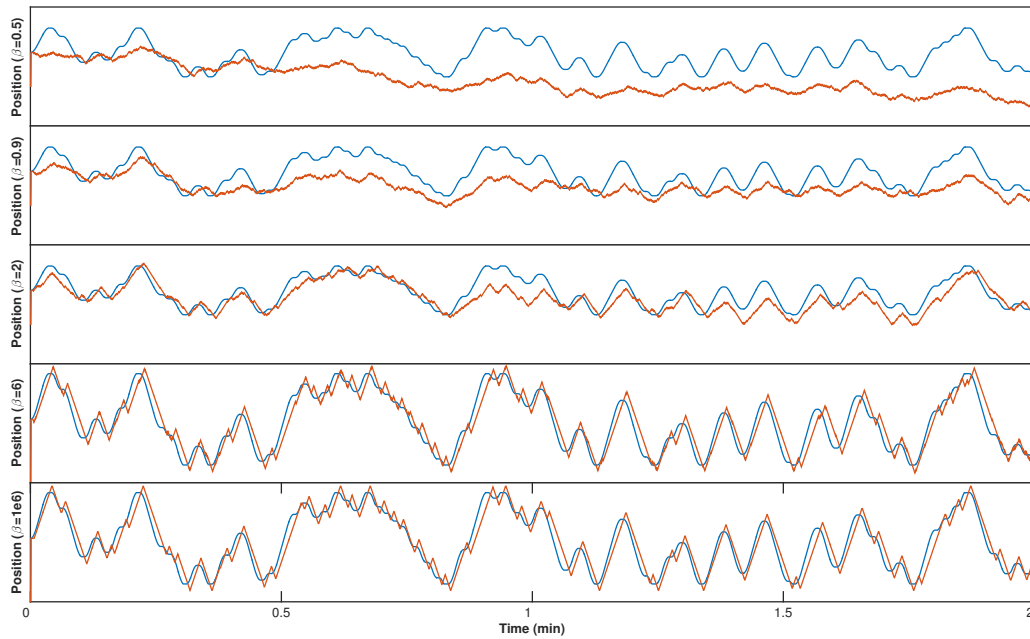
Fig. 5.14 Tracking trajectories of a LA-RI optimal controller for five levels of \beta : .5, .9, 2, 6 and 10^6 (from the top down) and actuation delay of 300 ms. Higher levels of \beta result in sharper policies enabling closer tracking.
