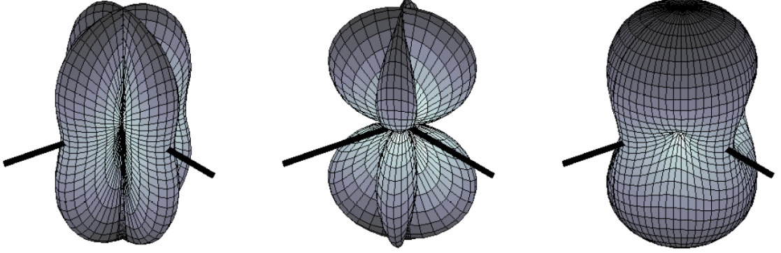
Figure 1.3: The antenna pattern of a GW interferometer. The antenna pattern is a measure of how sensitive a detector is in each direction. The black lines show the detector arms. The detectors have some sensitivity in almost all directions, and are most sensitive in the directions above and below the detector arms. Left is the antenna response for the plus polarization, middle is for the cross polarization and the right is for both polarizations. Figure reproduced from [54].
