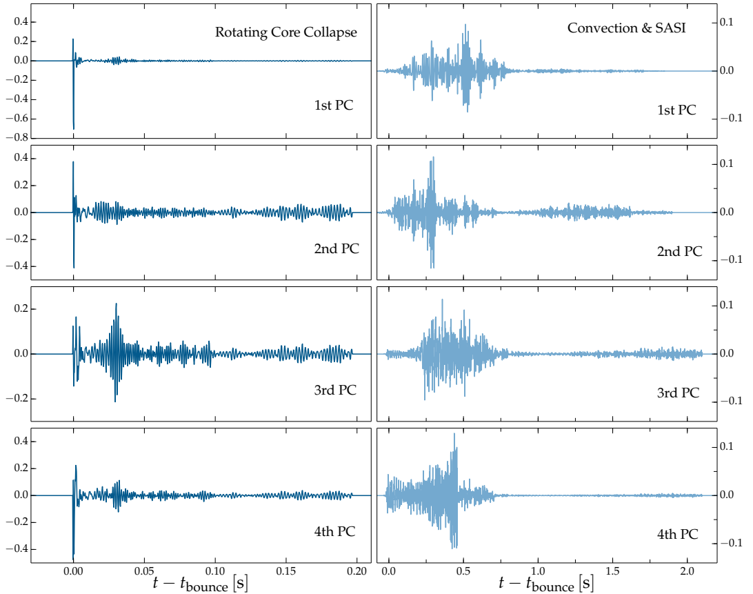
Figure 5.2: The first four three-dimensional PCs used to represent each explosion mechanism. For the magnetorotational signal model, 15 waveforms from Scheidegger et al. [114] are used. As for the two-dimensional magnetorotational model, the main feature of the PCs is the spike at core bounce. The neutrino mechanism signal model is made from a mixture of waveforms from Andresen et al. [156], Kuroda et al. [128] and Müller et al. [132]. The PCs are longer in duration than those produced with two-dimensional waveforms.
