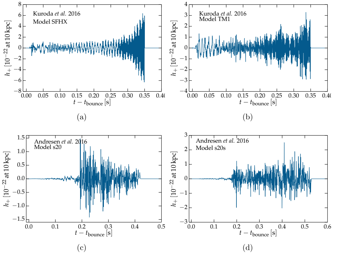
Figure 5.1: The h_+ time series of three-dimensional neutrino mechanism waveforms simulated by Kuroda et al. [128] and Andresen et al. [156]. (a) GWs from the simulation of a 15 M_{\odot} progenitor star with the SFHX EOS. (b) GWs from the simulation of a 15 M_{\odot} progenitor star with the TM1 EOS. (c) A 20 M_{\odot} progenitor star that does not explode, with strong low-frequency emission between 100 – 200 Hz. (d) GWs from the simulation of a 20 M_{\odot} progenitor star that successfully explodes. The amplitude is larger for the successful explosion than for the failed explosion.
