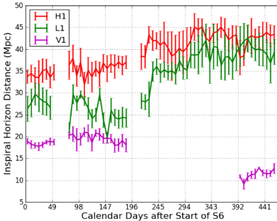
Figure 1.4: The inspiral horizon distance during the Initial LIGO and Virgo S6 and VSR2/3 runs. The average inspiral horizon distance is shown for each week with error bars that correspond to the standard deviation for that week. The Hanford detector was the most sensitive reaching distances of up to 45 Mpc towards the end of the science run. Figure reproduced from [60].
