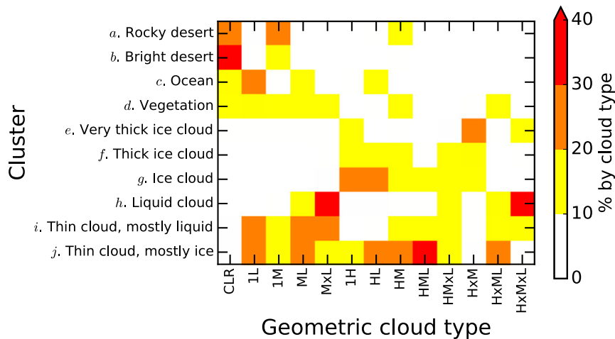
FIG. 8. The distribution of geometric cloud types and clear sky (CLR) among each of the 10 clusters presented in Fig. 1. Each cloud type is considered in isolation, such that each column adds up to 100%. The geometric cloud type classification allows for any combination of low- (L), mid- (M), or high-level (H) cloud separated at the pressure boundaries of 680 and 440 hPa. An “x” between letters denotes that the cloud extends across the pressure levels.
