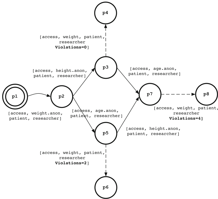
Fig. 4 Pseudonymization risk analysis output
