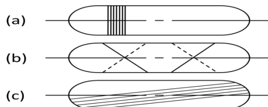
Figure 1: Filament-winding-molding method, (a) parallel winding method, (b) spiral winding method and (c) level winding method
