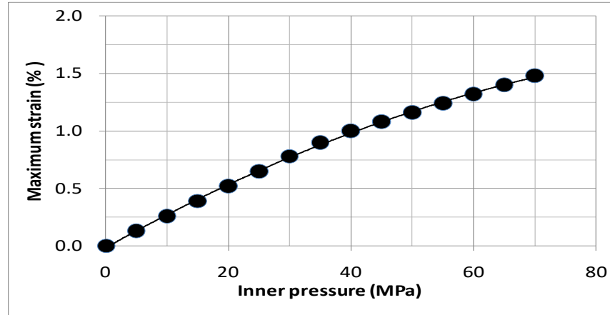
Figure 8: Relation between the maximum strain analysis values and the internal pressure around the CFRP tank cap part
