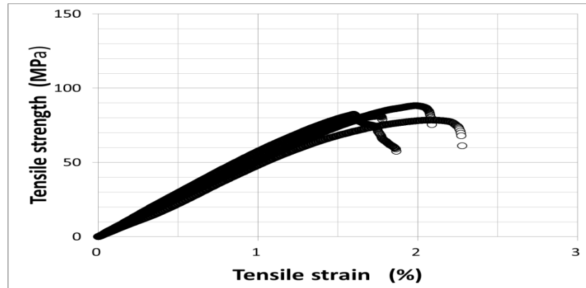
Figure 5: Relation between the stress and the strain to have gotten from the tension test (fiber rolling angle is \pm 45^\circ )
