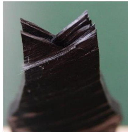
Figure 6: fracture surface of a specimen after tension test (fiber rolling angle is \pm 45^\circ )
