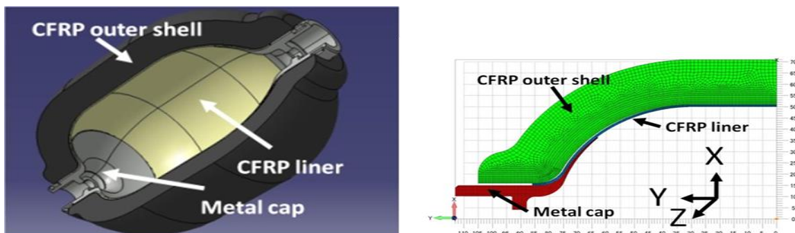
Figure 7: Finite-element-method analysis model of CFRP container fabricated by FW method
