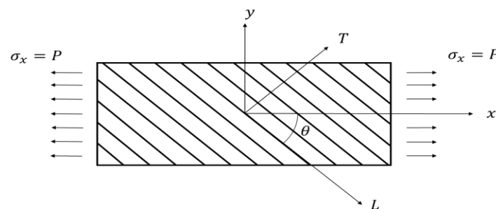
Figure 2: Orthotropic anisotropic board on which load acted in x-direction
