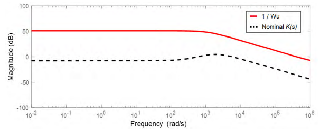
FIGURE 6. K(s) of the nominal system.
