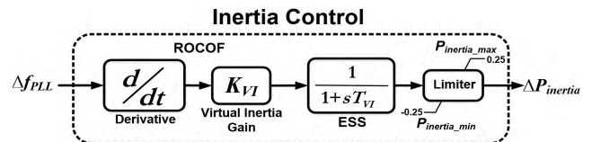
FIGURE 3. A dynamic structure of the virtual inertia control.
