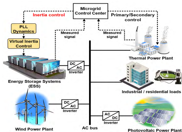
FIGURE 1. A schematic diagram of the islanded microgrid.
