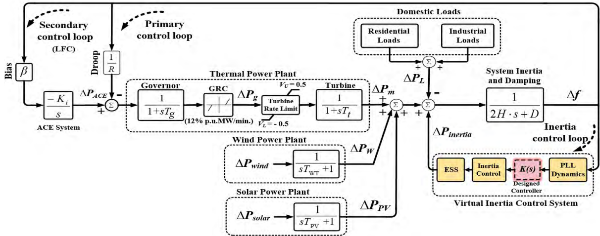
FIGURE 2. A dynamic structure of the microgrid for frequency stability analysis.
