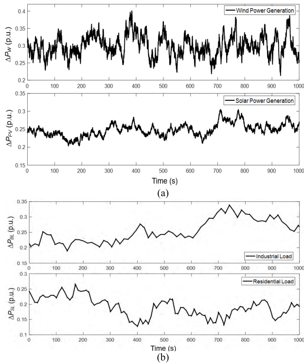
FIGURE 11. Severe disturbances for scenarios C and D: (a) Renewable power generations in the presence of high wind speed and solar irradiation, (b) Industrial and residential load demand patterns.
