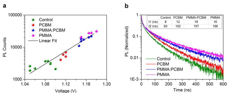
Fig. 3 a ) Logarithmic plot of PL intensity vs V_{oc} . b ) Time-resolved photoluminescence (TRPL) decay measurements for the perovskite thin films on FTO/C-In-TiO x /m-TiO 2 substrates with/without PCBM, PMMA:PCBM (1:3) or PMMA passivation layer.
