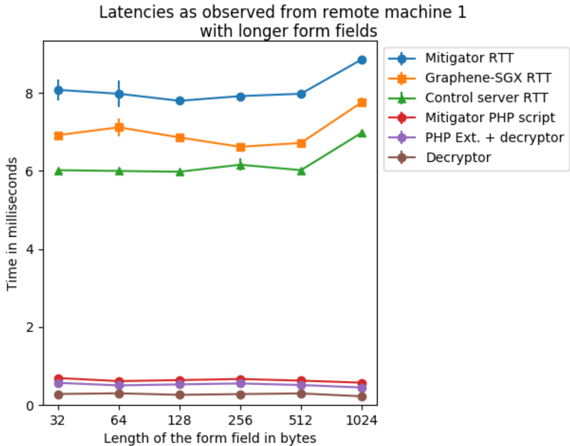
Figure 6.3: Measurement of server-side latency from remote machine 1 as the size of a form field increases: the length of a single form field was doubled in steps from 32 to 1024 and we measured the round-trip times (RTT) from remote machine 1 for each of the Mitigator, Graphene-SGX, and control servers, and the averages, over 50 requests for each form field length, are plotted in blue, orange, and green respectively. For the Mitigator server, we measured the total wall clock time spent within the PHP script, the total time spent within the PHP extension and the decryptor enclaves and the time spent within the decryptor enclave and the corresponding averages are plotted in red, light purple, and brown respectively. The standard error bars for most values in this dataset are too small to be seen on this graph.
