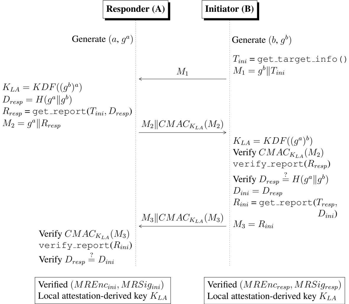
Figure A.2: Two-sided local attestation-based key exchange protocol used in Intel’s SGX SDK and in Mitigator that shows how trusted Intel SGX instructions can be used to perform a bidirectional local attestation resulting in a secure channel between enclaves. The functions shown in typewriter font are executed through trusted SGX instructions, as shown in Figure A.1. As per the output of the get_report() function in that figure, the reports R_{ini} and R_{resp} always include information about their own SECS page in their report bodies, that is, T_{ini} || MRSig_{ini} and T_{resp} || MRSig_{resp} respectively.
