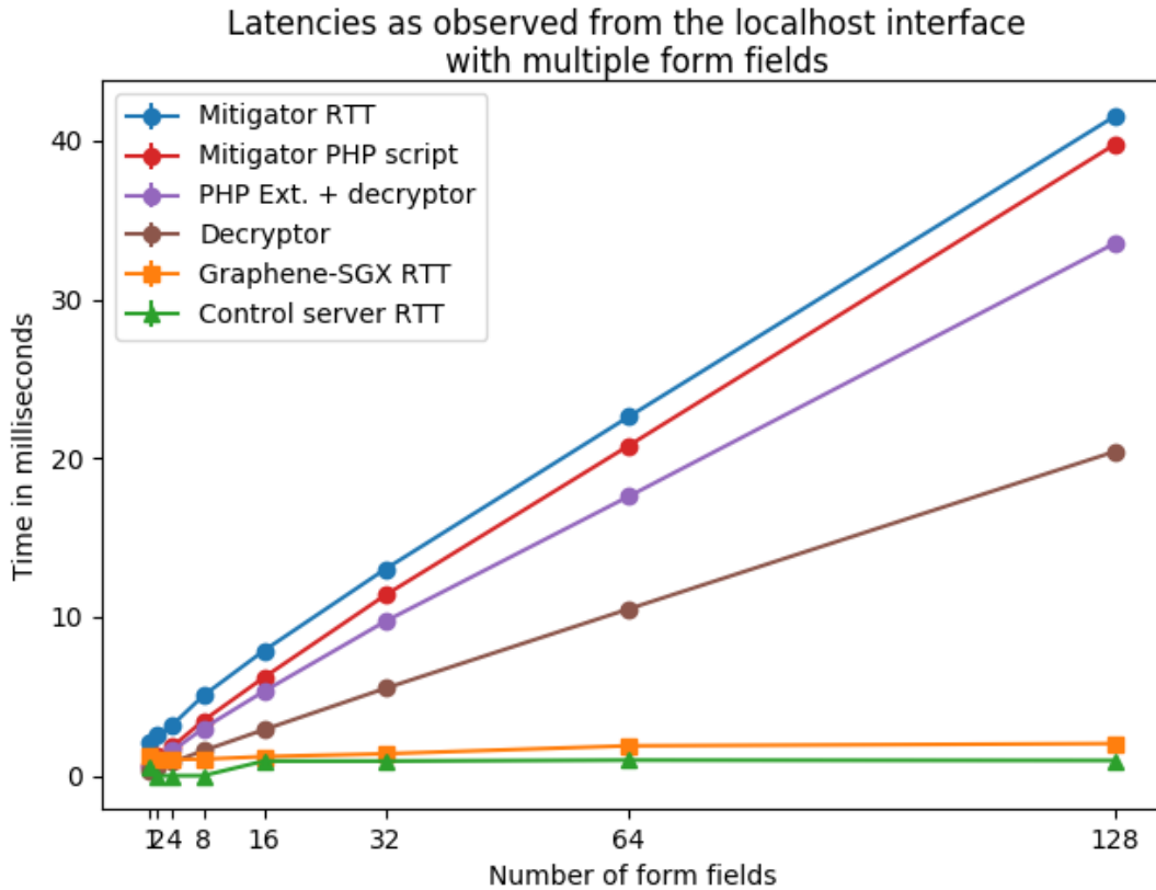
Figure 6.2: Measurement of server-side latencies from the localhost interface as the number of form fields increases: starting from 1, the number of form fields was doubled in steps up to 128, and we measured the round-trip times (RTT) from the localhost interface for each of the Mitigator, Graphene-SGX, and control servers, and the averages, over 50 requests for each number of form fields, are plotted in blue, orange, and green respectively. For the Mitigator server, we measured the total wall clock time spent within the PHP script, the total time spent within the PHP extension and the decryptor enclaves, and the time spent within the decryptor enclave and the corresponding averages are plotted in red, light purple, and brown respectively. The standard error bars for this dataset are too small to be seen on this graph.
