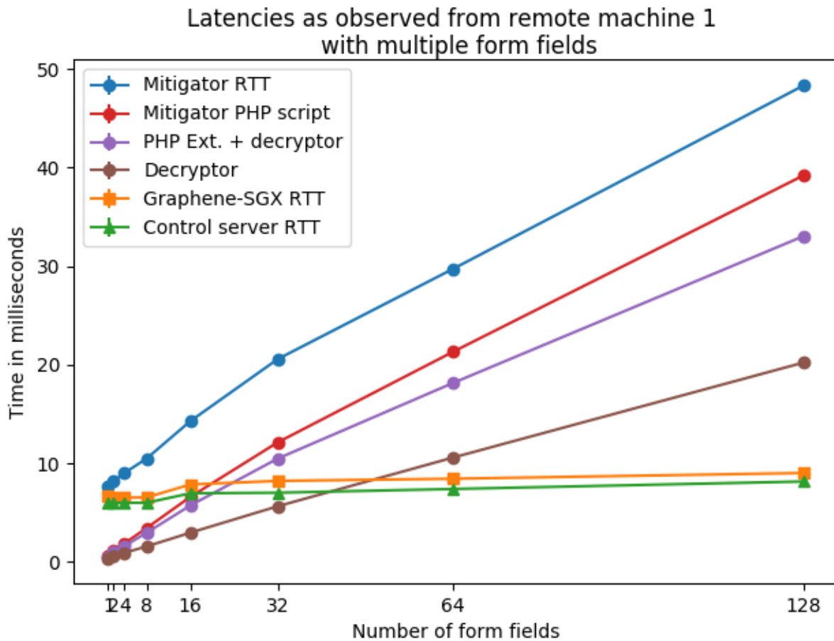
Figure 6.4: Measurement of server-side latencies from remote machine 1 as the number of form fields increases: starting from 1, the number of form fields was doubled in steps up to 128, and we measured the round-trip times (RTT) from remote machine 1 for each of the Mitigator, Graphene-SGX, and control servers, and the averages, over 50 requests for each number of form fields, are plotted in blue, orange, and green respectively. For the Mitigator server, we measured the total wall clock time spent within the PHP script, the total time spent within the PHP extension and the decryptor enclaves, and the time spent within the decryptor enclave and the corresponding averages are plotted in red, light purple, and brown respectively. The standard error bars for this dataset are too small to be seen on this graph.
