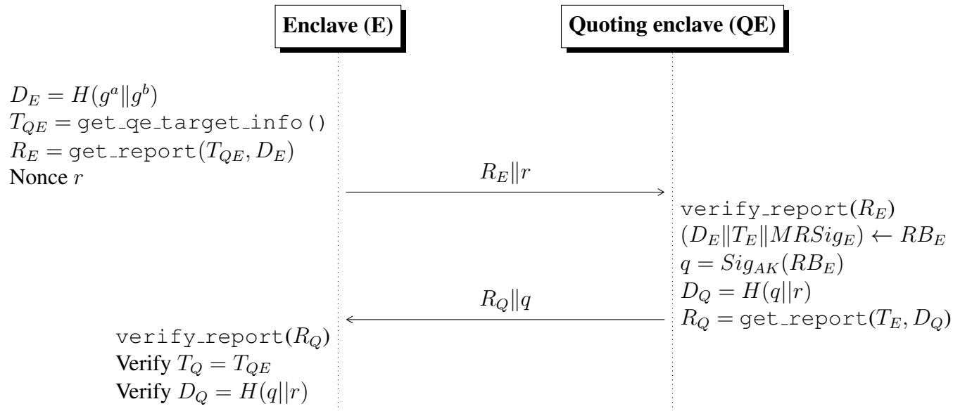
Figure A.4: This sequence diagram shows a custom local attestation protocol between the enclave E and another enclave with a special interface, known as the Quoting Enclave (QE), which occurs during remote attestation. The Quoting Enclave signs the report body of a local attestation report with an attestation key AK , such that the client can query Intel to verify the signature on the report body. We remark that the report body RB_E in the report R_E contains the report data D_E as well as the enclave and signer measurements and other enclave attributes ( T_E \| MR\text{Sig}_E ). The signed report body is known as a quote and is denoted by q in this diagram. We use the three functions shown in Figure A.1 and introduce another function named get_qe_target_info() , which returns the target information of the quoting enclave to the calling enclave.
