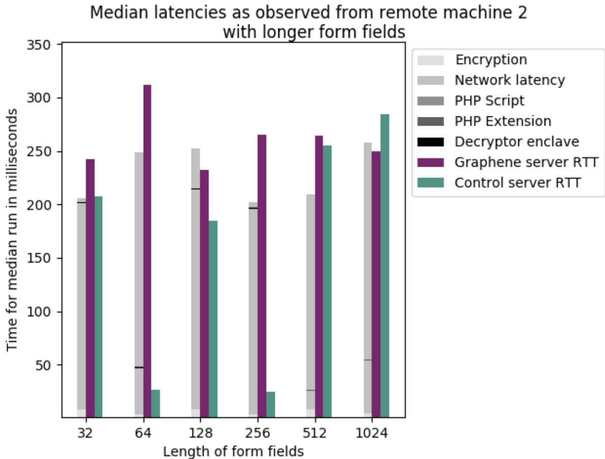
Figure 6.5: Distribution of time in median runs as the length of a single form field sent in the request varies: on doubling the length of the form field sent in each request, the client-side encryption time (lightest grey) and time spent in each of the Mitigator server-side components (darker shades of grey) are plotted for the median run for the given length of the form field. The median runs for the Graphene-SGX and control servers are also plotted in purple and teal respectively.
