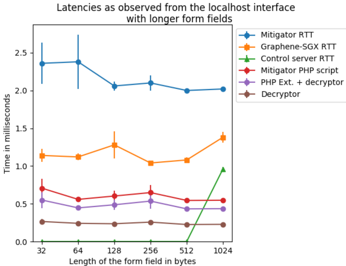
Figure 6.1: Measurement of server-side latency from the localhost interface as the size of a form field increases: the length of a single form field was doubled in steps from 32 to 1024 and we measured the round-trip times (RTT) from the localhost interface for each of the Mitigator, Graphene-SGX, and control servers, and the averages, over 50 requests for each form field length, are plotted in blue, orange, and green respectively. For the Mitigator server, we measured the total wall clock time spent within the PHP script, the total time spent within the PHP extension and the decryptor enclaves and the time spent within the decryptor enclave and the corresponding averages are plotted in red, light purple, and brown respectively.
