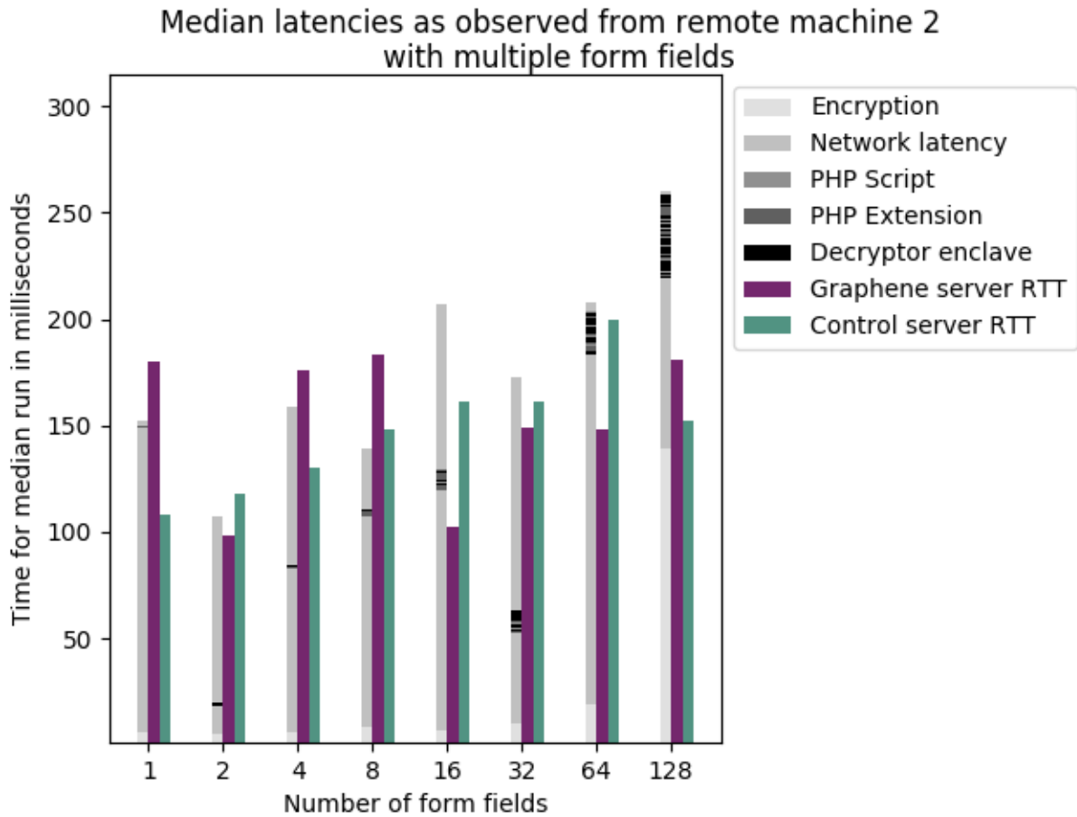
Figure 6.6: Distribution of time in median runs as the number of form fields sent in the request varies: on doubling the number of form fields sent in each request, the client-side encryption time (lightest grey) and time spent in each of the Mitigator server-side components (darker shades of grey) are plotted for the median run for the given number of form fields. The median runs for the Graphene-SGX and control servers are also plotted in purple and teal respectively.
