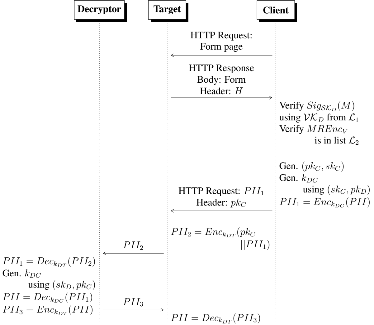
Figure 4.4: This figure captures the runtime stage of Mitigator. Prior to this stage, the target enclave should have conducted local attestation with the decryptor enclave resulting in the symmetric key k_{DT} being established between the two enclaves. The target enclave should have obtained the signed token H from the decryptor enclave over the secure channel established with it. This token has the form shown in Figure 4.3. We remark that the target enclave should send the token H in the response header of all HTTP responses to requests for an HTML form page. In order to verify the integrity of the token H , the client obtains the decryptor enclave’s long-term verification key \mathcal{VK}_D from list \mathcal{L}_1 and the verifier enclave’s expected enclave measurement from list \mathcal{L}_2 .
