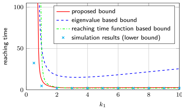
Fig. 4. Comparison of reaching time bounds with k_2 = 1 and initial state \mathbf{x}_0 = [1 \quad 1]^T , and simulation results with \delta_2 = L [x_1]^0 as a function of the parameter k_1 for K = 0 , L = 0.5 .
