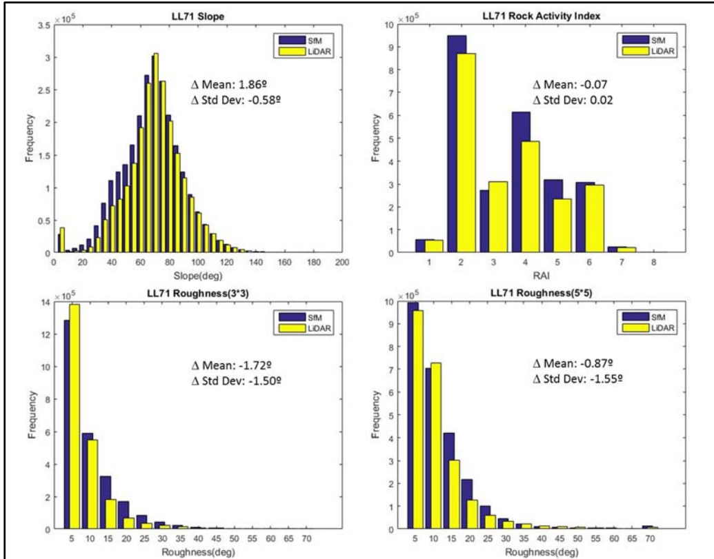
Figure 15 - Site LL71 Histogram comparison of DSM properties
