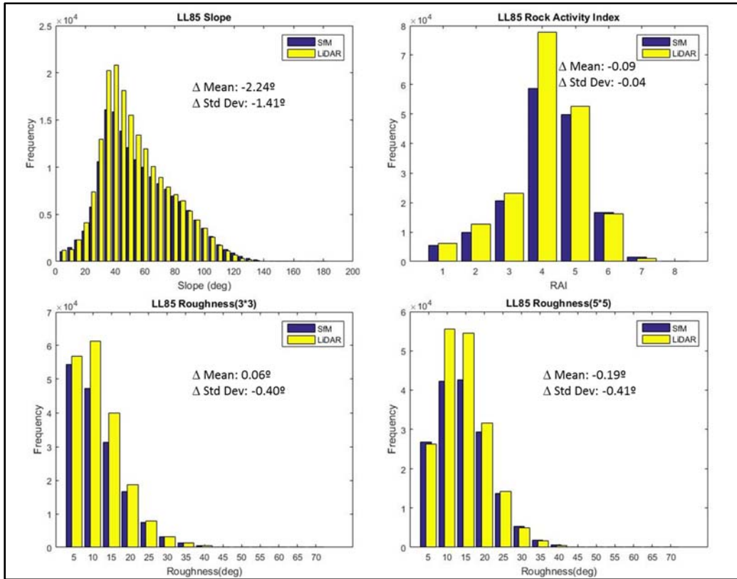
Figure 16 - Site LL85.5 Histogram comparison of DSM properties
