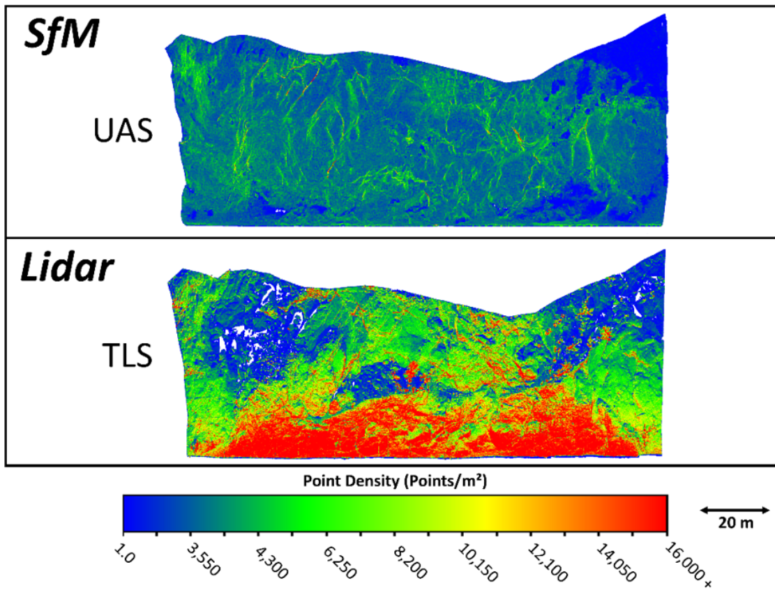
Figure 10 - Point densities for both surface models
