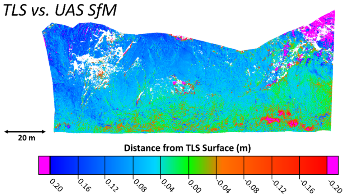
Figure 11 - Difference of the SfM from the TLS models
