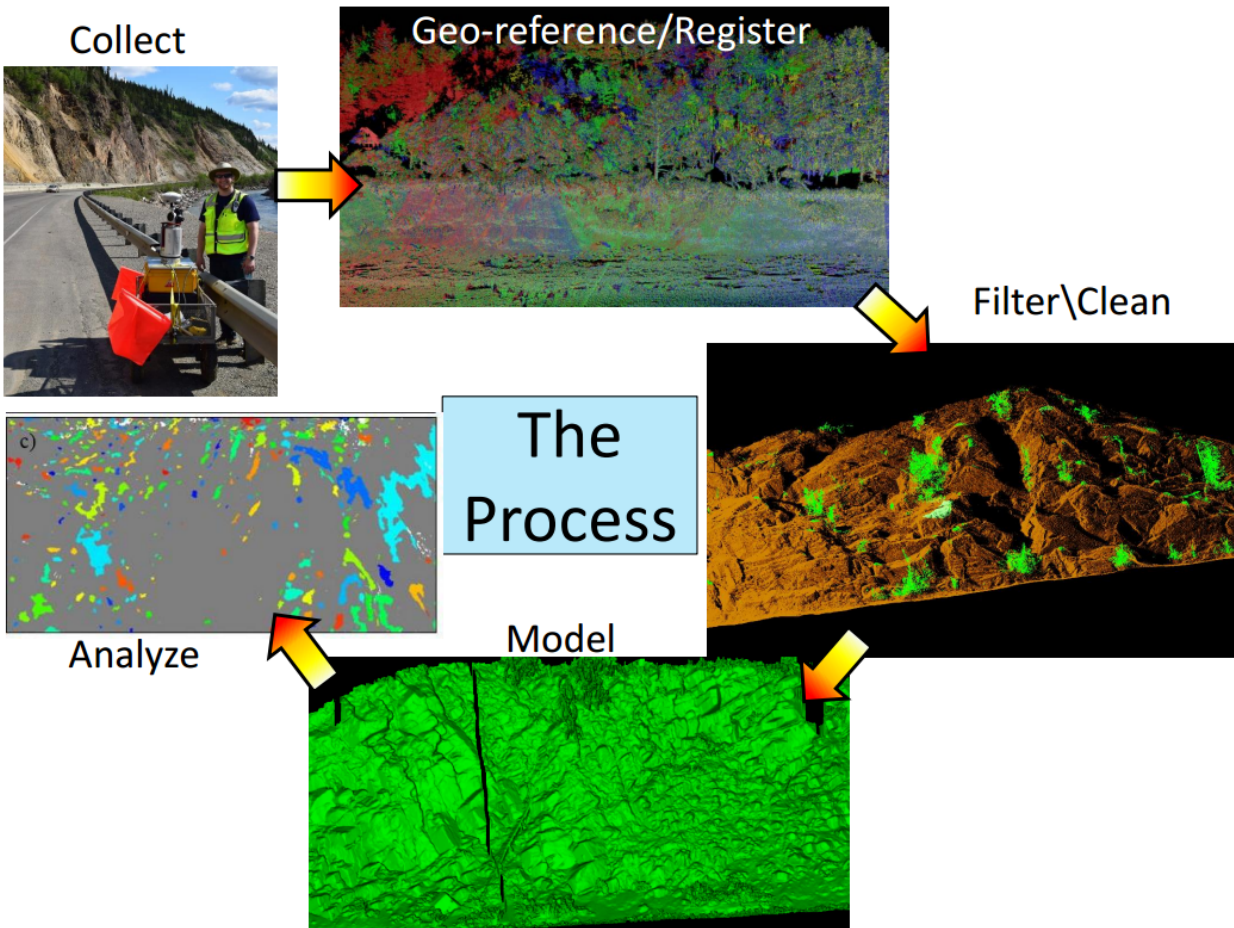
Figure 2 - Overview of workflow implemented for this project
