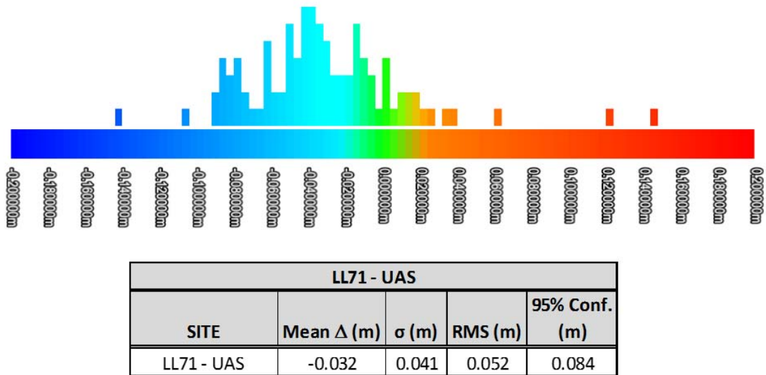
Figure 13 - Statistics from the UTIC SfM surface model
