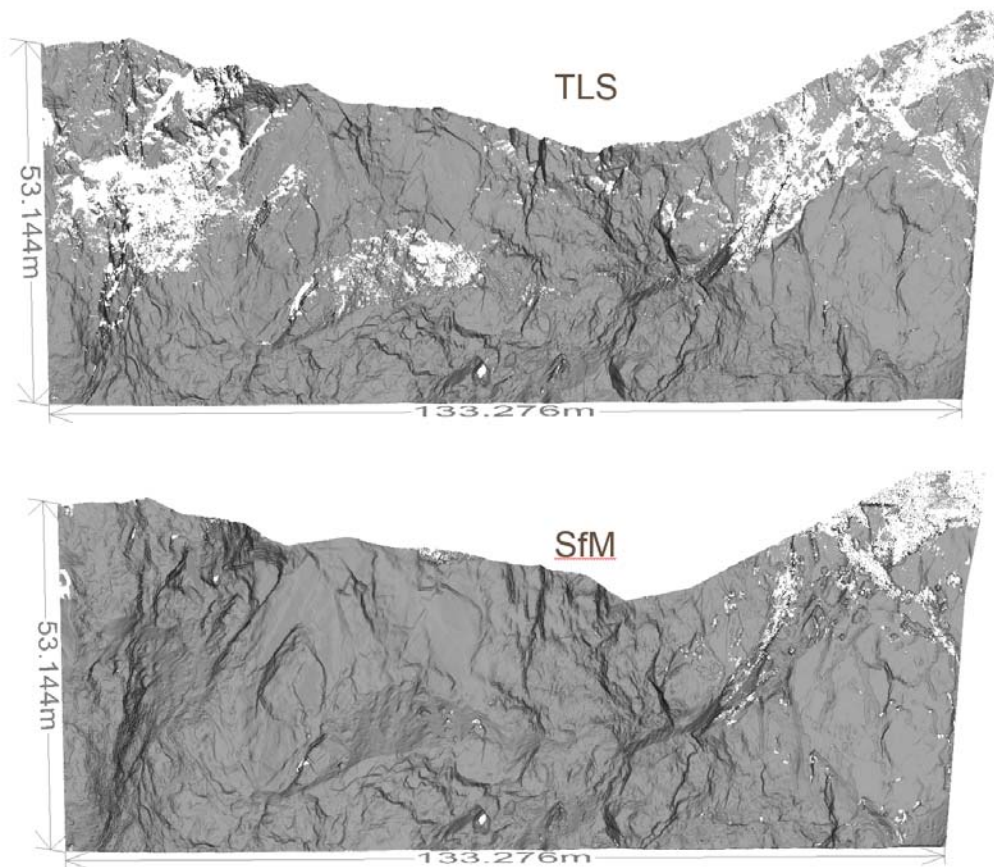
Figure 9 - The TLS and SfM surface models, with white patches indicating data voids
