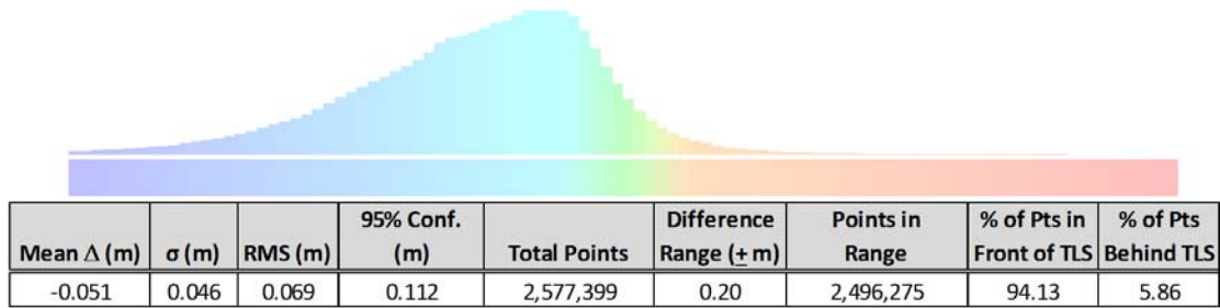
Figure 12 - Statistics differencing the two DSM
