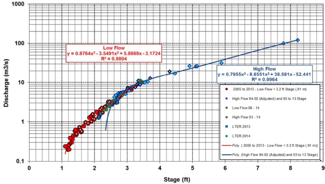
Upper Kuparuk River 1994 to 2002 Rating Curves Adjusted High Flow and Upper Kuparuk River 2005 to 2014 New Rating Curve To convert Tylers 2014 BM to old staff gauge add 0.23 ft.
