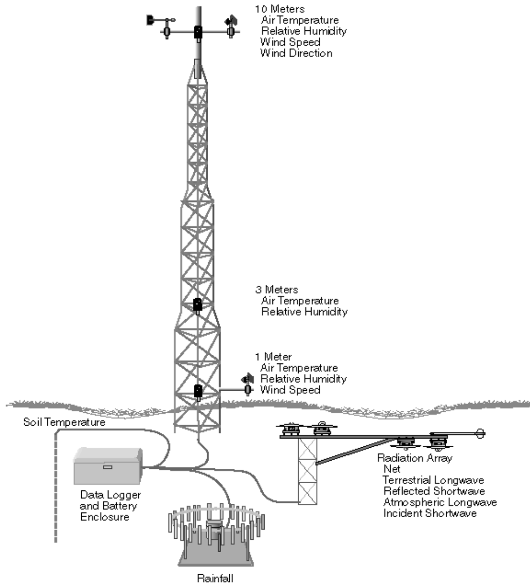
Figure 1. Typical 10 m tower meteorological station. Innavaik, Upper Kuparuk, and Franklin Bluffs are 10 m towers.
