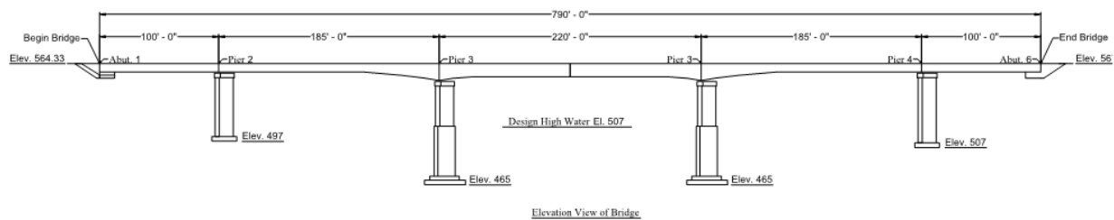
Figure 2.1 Elevation: Chulitna River Bridge
