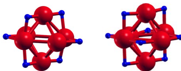
Fig. 9. Lowest energy structures of \text{Co}_6 with six and eight chemisorbed H atoms.
