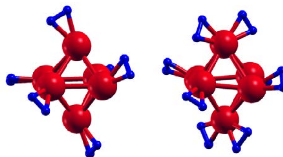
Figure 14. Molecular adsorption of six and eight H_2 molecules on Co_6 .
