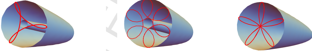
Figure 2: Three plots of the classical trajectories (4.24) of the classical FD system (in red) with the surfaces of the effective potentials. On the left \{\gamma = 1/3, p + q = 3, \ell = 96, \alpha_0 = 10, \beta_0 = 14, \theta_1 = \theta_2 = 0\} , on the center \{\gamma = 2/3, p + q = 6, \ell = 125, \alpha_0 = 10, \beta_0 = 15, \theta_1 = 2, \theta_2 = 3\} , and on the right \{\gamma = 1/5, p + q = 5, \ell = 0, \alpha_0 = 12, \beta_0 = 12, \theta_1 = 2, \theta_2 = 1\} .
