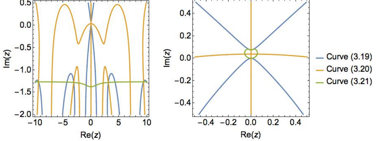
Figure 2: On the left, for some values of the parameters ( v_0 = -2 , v_1 = 4 , w_0 = -1 , w_1 = 3 and q = 1/2 ), the typical behavior of the curves (3.19)–(3.21) is plotted. The intersections between the blue and orange curves (the values of z such that the real and imaginary parts of \Delta(z) are simultaneously zero) are seen as discrete points, placed on the compatibility condition curve (green). Remark that there is an infinity number of such solutions on the lower part of the complex plane, appearing in pairs z = \pm z_{r,n} - iz_{i,n} , z_{r,n}, z_{i,n} > 0 , n = 1, 2, \dots , corresponding accordingly to resonances in the spectrum; in addition, there is also one imaginary solution with positive imaginary part z_0 = iz_{i,0} . On the right, a zoom of the same plot near the origin is shown. One may observe a bound state in the upper intersection. The lower intersection, however, happens exactly at the origin and it is not a meaningful physical solution.
