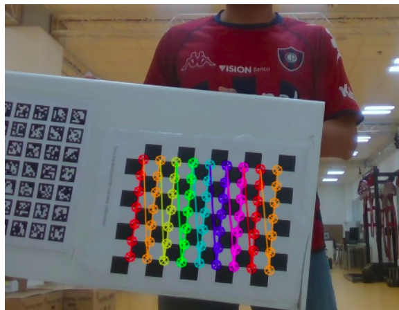
Figure 4.4: Overview of a 7 \times 9 checkerboard calibration grid
