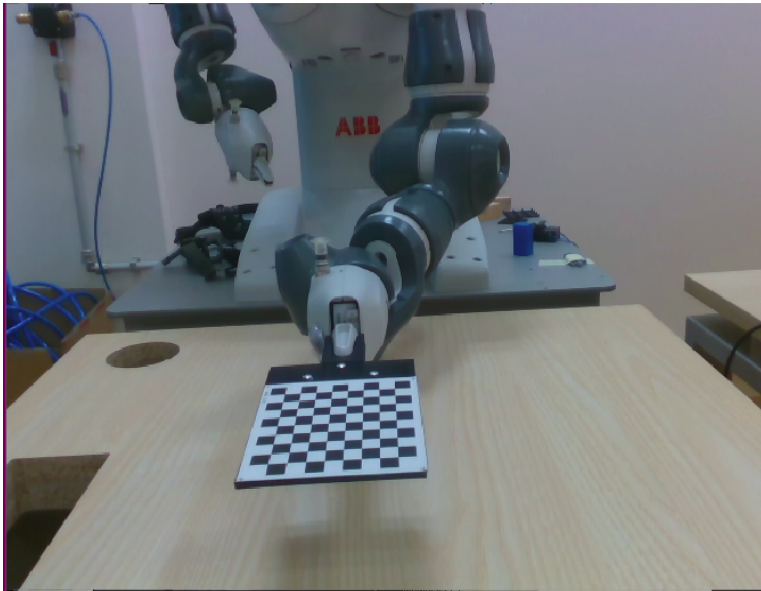
Figure 4.6: An 8 \times 9 Checkerboard Calibration Target fixed on a custom-made plate
