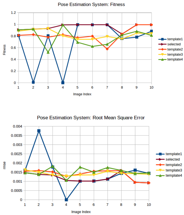
Figure 6.23: Results: Pose Estimation System with the RealSense D-415 Camera
