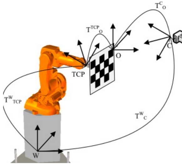
Figure 4.1: Overview of the camera pose estimation system. The system estimates the pose of the camera frame relative to the world frame (also known as robot base frame). Image from [22].
