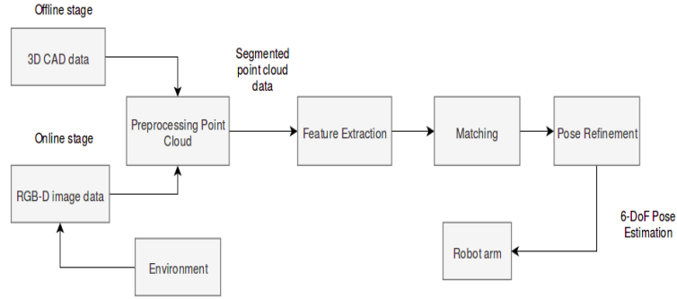
Figure 5.1: General architecture of proposed pose estimation pipeline
