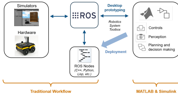
Figure 3.6: A ROS Overview
