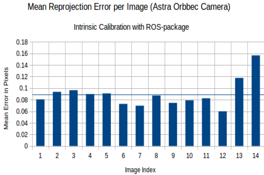
Figure 6.3: Mean Reprojection Error per Image with the ROS Method (Astra Orbbec Camera)
