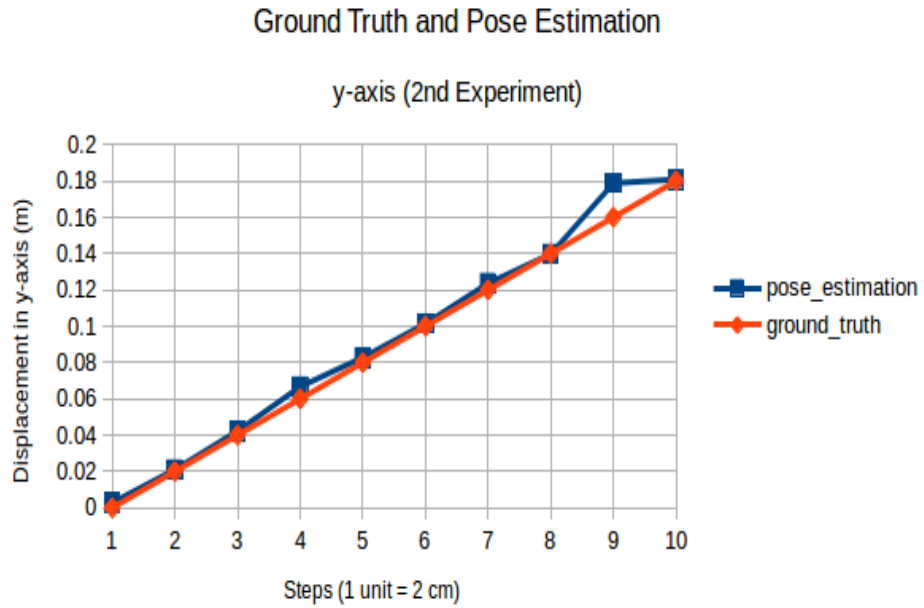
Figure 6.14: Ground Truth and Pose Estimation: y-axis (2 nd Experiment, Astra Camera)
