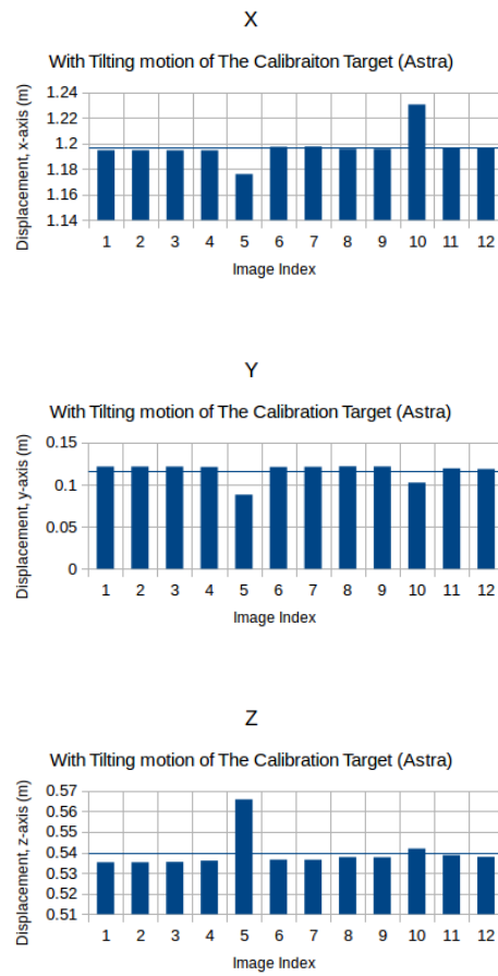
Figure C.2: Eye-To-Hand Result with Tilting Motion of the Calibration Plate (Astra Camera)
