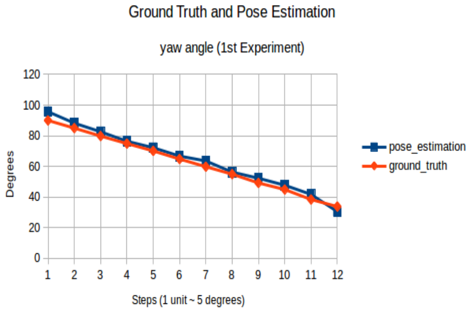
Figure 6.12: Ground Truth and Pose Estimation: yaw angle (1 st Experiment, Astra Camera)
