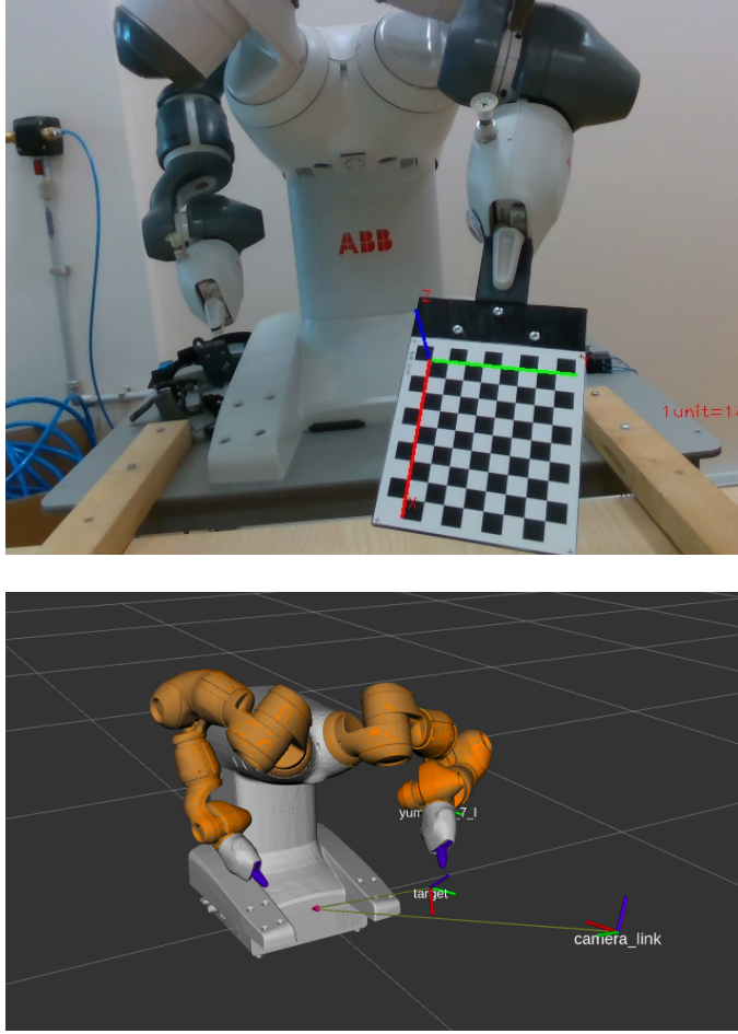
Figure 6.8: System setup and Visualization in Rviz of the Validation Test with Tilting Motion.
