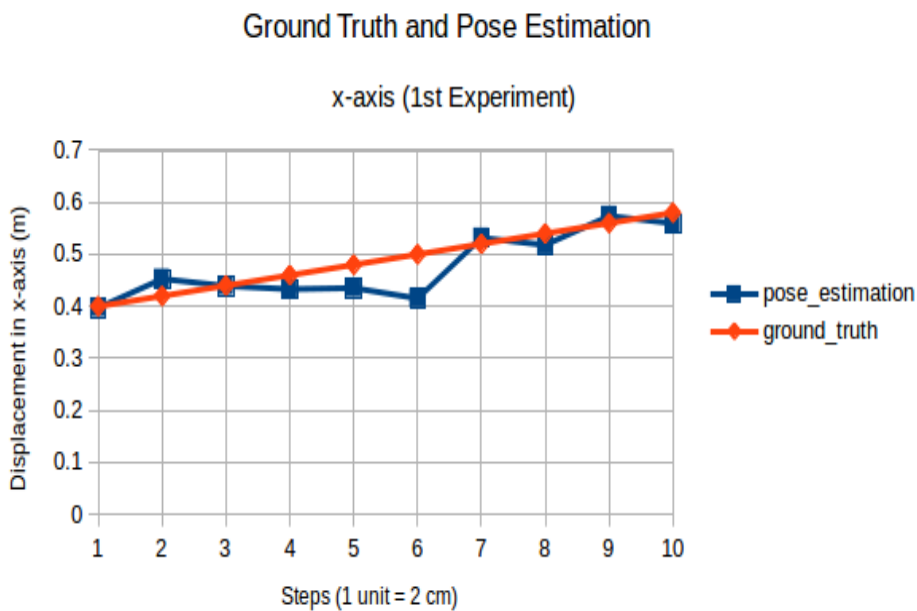
Figure 6.10: Ground Truth and Pose Estimation: x-axis (1 st Experiment, Astra Camera)
