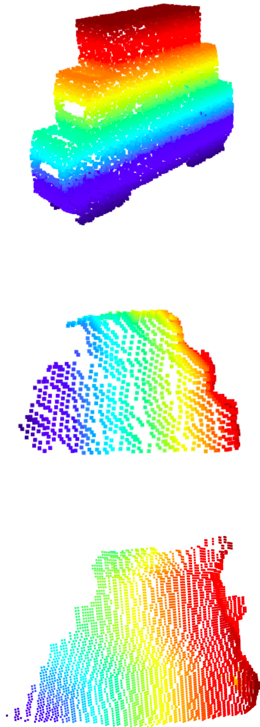
Figure 6.19: Point Cloud Sources: CAD model, Astra Camera and RealSense D-435 Camera from top to bottom
