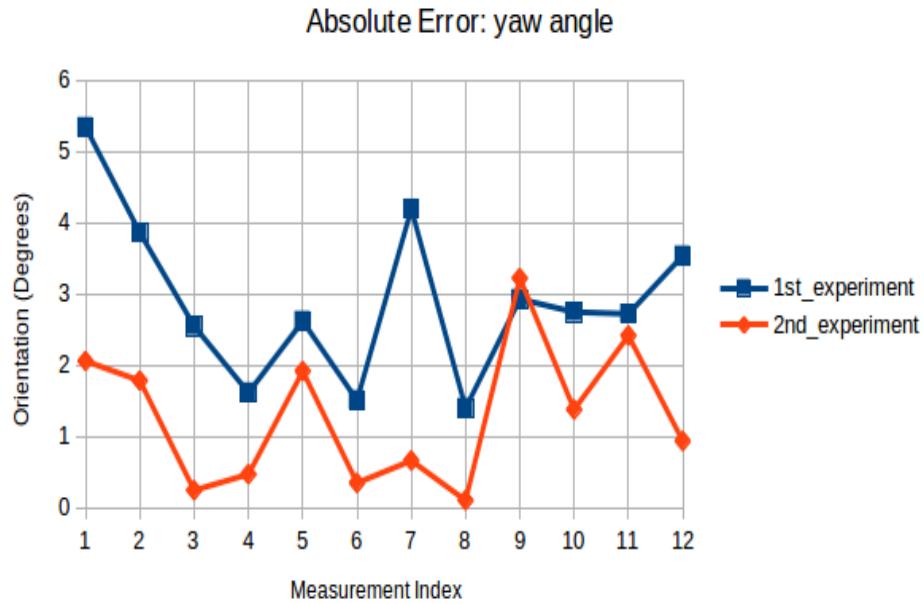
Figure 6.18: Absolute Error: yaw angle
