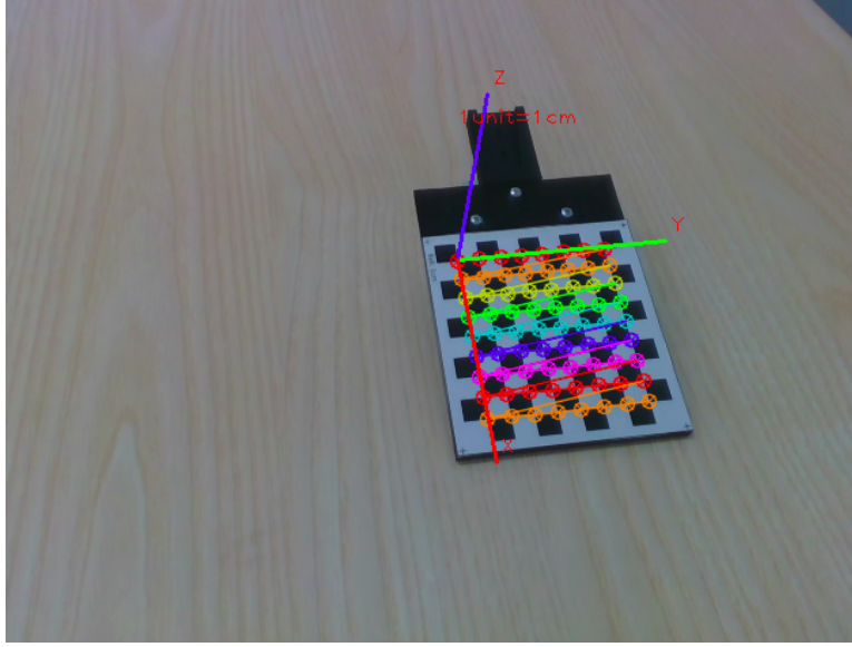
Figure 4.7: Visualization of the 3D world coordinates system projected onto the 2D image plane
