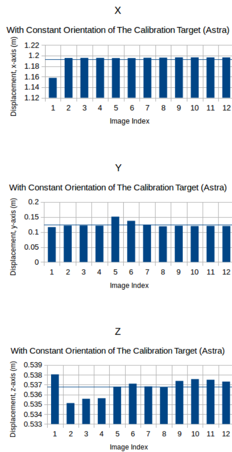
Figure C.1: Eye-To-Hand Result with a Constant Orientation of the Calibration Plate (Astra Camera)
