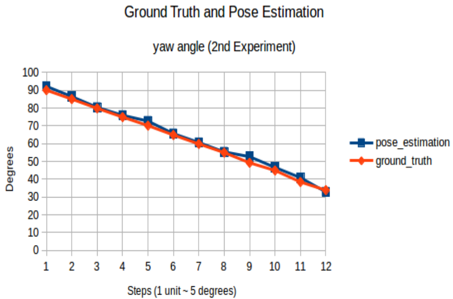
Figure 6.15: Ground Truth and Pose Estimation: yaw angle (2 nd Experiment, Astra Camera)
