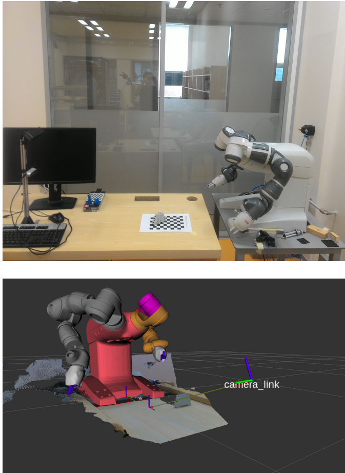
Figure 6.2: Overview of the Validation System: Checkerboard placement and Visualization in Rviz simulator.
