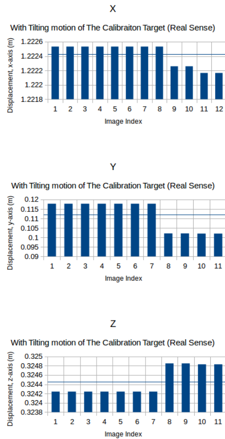
Figure C.4: Eye-To-Hand Result with Tilting Motion of the Calibration Plate (RealSense Camera)
