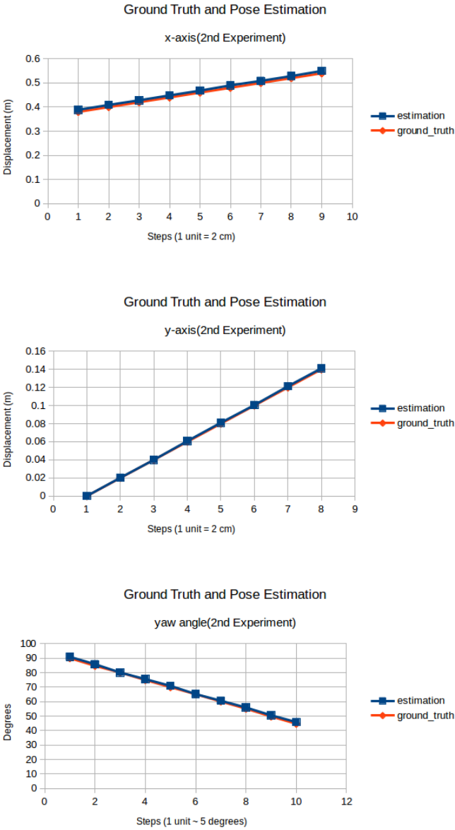
Figure 6.21: Ground Truth and Pose Estimation (2 nd Experiment, RealSense D-415)
