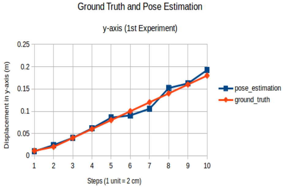
Figure 6.11: Ground Truth and Pose Estimation: y-axis (1 st Experiment, Astra Camera)
