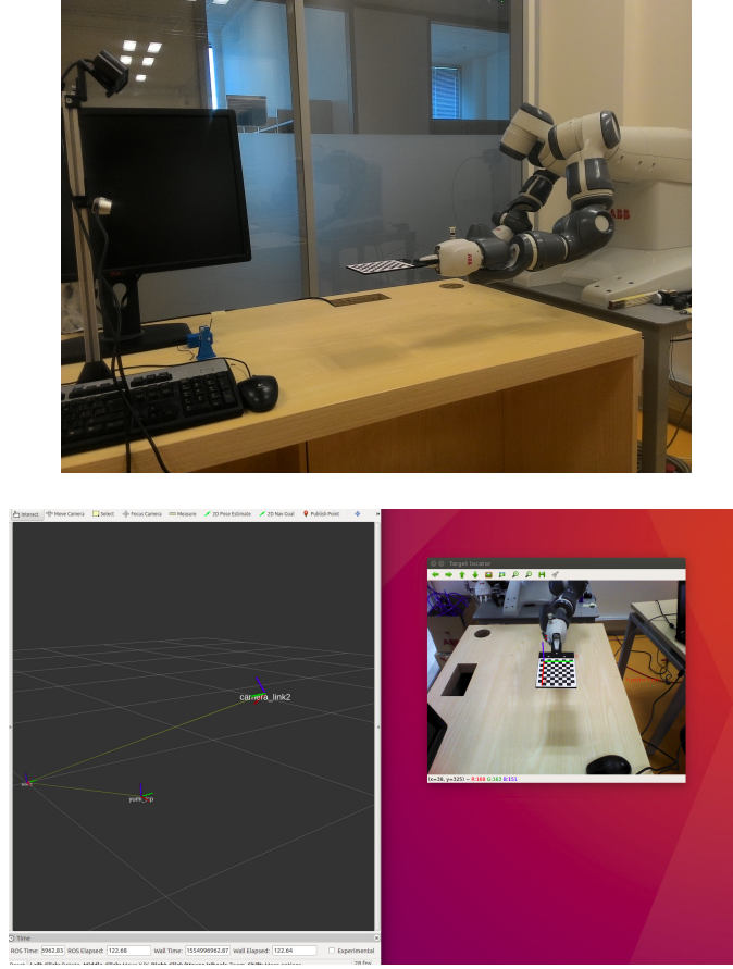
Figure 6.7: System setup and Visualization in Rviz of the Validation Test with a Constant Orientation.
