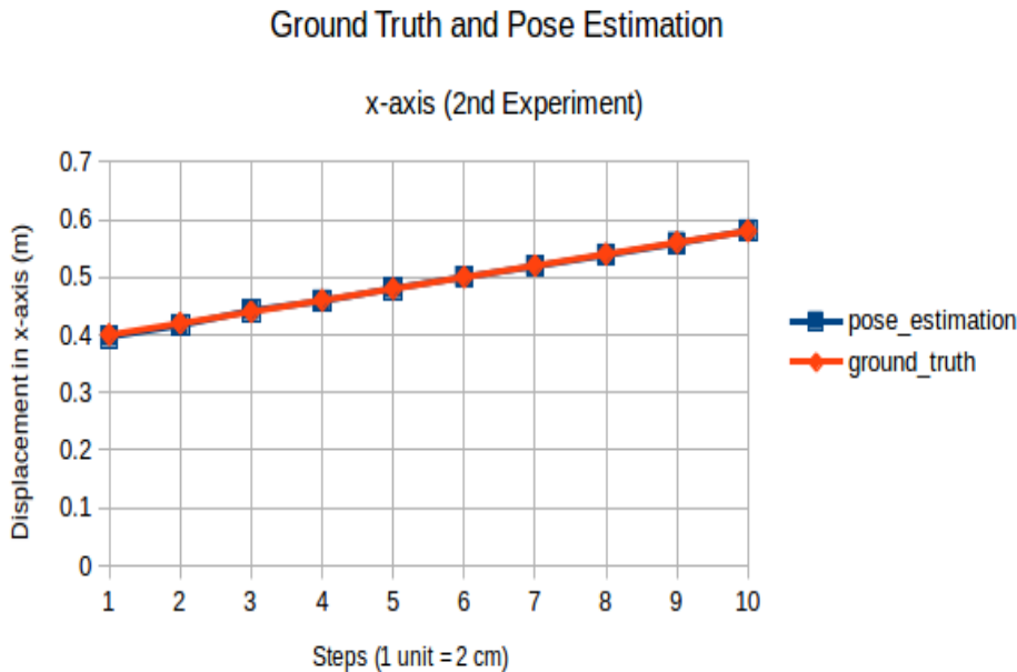
Figure 6.13: Ground Truth and Pose Estimation: x-axis ( 2^{nd} Experiment, Astra Camera)
