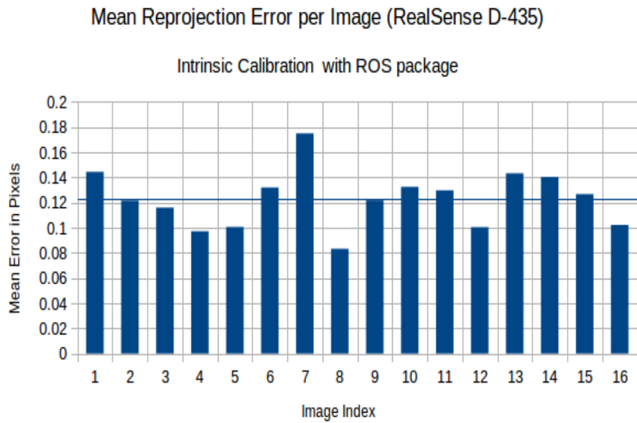
Figure 6.4: Mean Reprojection Error per Image with the ROS Method (RealSense D-435)
