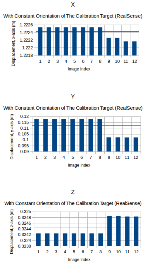
Figure C.3: Eye-To-Hand Result with a Constant Orientation of the Calibration Plate (RealSense)
