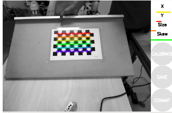
Figure 4.2: Overview of the intrinsic calibration based on industrial calibration ROS package with a 6 \times 9 checkerboard calibration target
