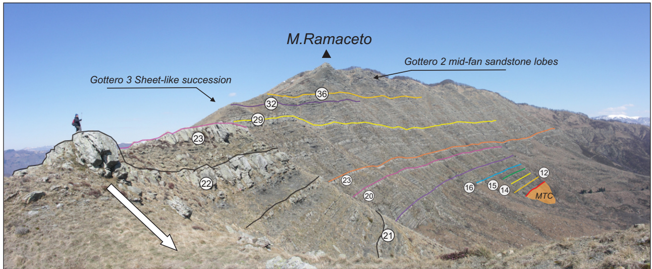
Fig.13 - Exposure of the upper stratigraphic part of Gottero Sandstone in the Mt. Ramaceto area. Note the succession is tectonically inverted. Numbers refer to key horizons highlighted in Plate 2. Orange colour represents the outcrop of the stratigraphically overlying Gaiette mass transport complex unit (MTC).
