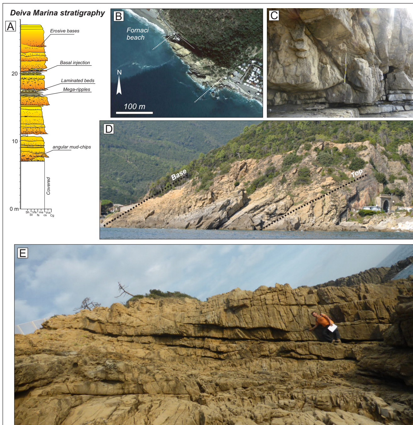
Fig. 8 - Deiva Marina outcrops and log. A) Stratigraphic log and main facies features. B) Geographic position of Deiva Marina exposure from Google maps. C) Convex-downward scour at the base of an amalgamated sandstone package. D) Deiva Marina exposure seen from the sea. E) Rotated field photograph showing cut-and-fill feature at the base of an amalgamated sandstone bed.
