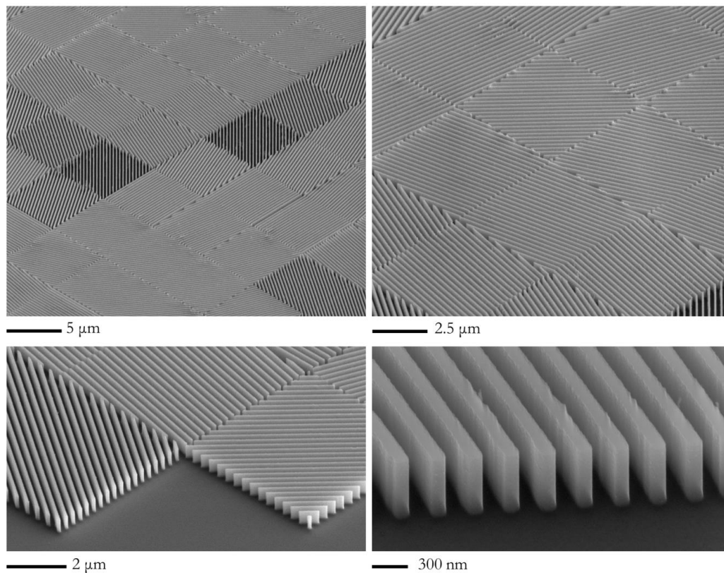
Figure 4. SEM inspections of the fabricated PBOE on a silicon substrate. Grating period \Lambda = 290 nm, duty cycle 0.5, thickness: 535 nm, pixel size: 6.125 \mu\text{m} , 16 rotation angles.
