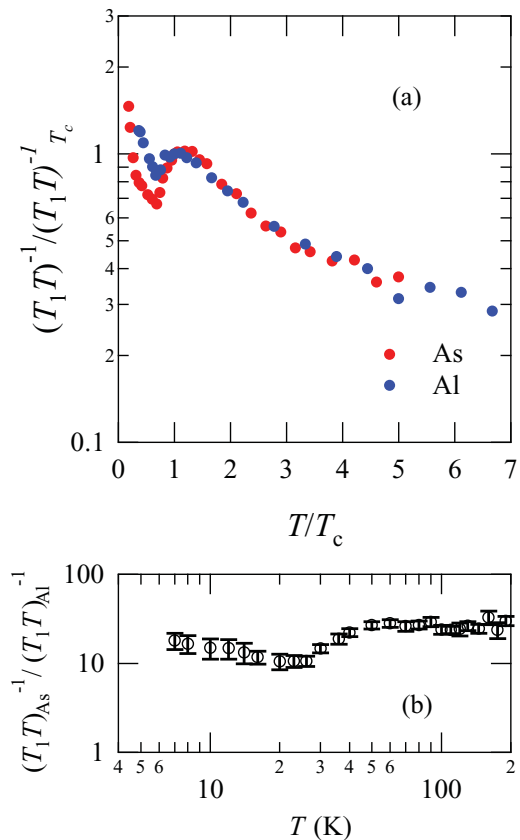
FIG. 4. (Color online) (a) Plot of 1/T_1 T versus T normalized by those at T_c . (b) The ratio of (1/T_1 T)_{\text{As}} / (1/T_1 T)_{\text{Al}} . The values are almost the same except for the temperature range between 20 and 40 K corresponding to T_c values at zero field and 20.8 kOe.
