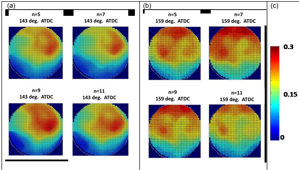
Figure 9: Typical reconstructed distributions of liquid fuel spray in four engine cycles, each cycle numbered ( n ) within a single fuelled sequence, at given crank angles after exhaust Top Dead Centre ( =0^\circ\text{CA} ), (a) at 143^\circ\text{CA} , and (b) at 159^\circ\text{CA} . The colour scale (arbitrary units) is shown in part (c), and is fixed for all images in this Figure.
