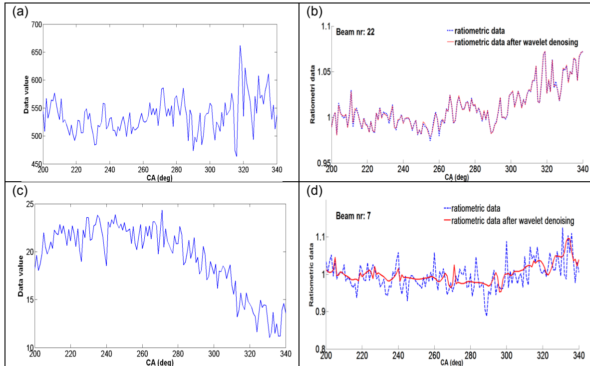
Figure 4: Examples of application of Wavelet Denoising (WD): (a) raw single-wavelength data indicating a high-quality beam (#22); (b) DWR data for beam 22 before and after WD; (c) raw single-wavelength data indicating a poor-quality beam (#7); (d) DWR data for beam 7 before and after WD.
