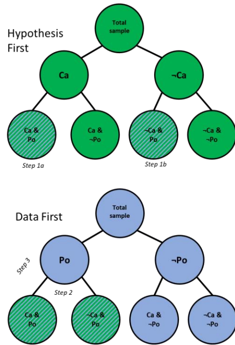
Figure 3. 'Hypothesis First' and 'Data First' tree diagram representations of the medical diagnosis problem.
