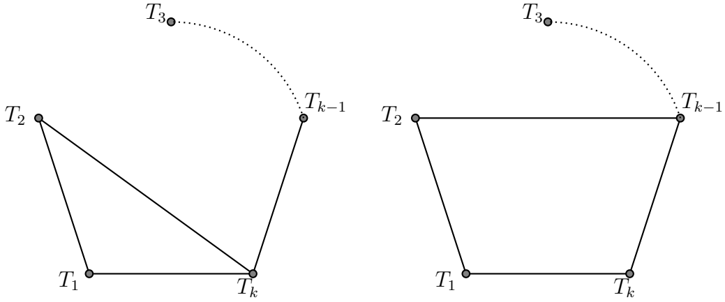
Figure 5. Modifications G_1 and G_2 for graph G
