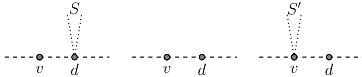
Figure 3. the graph G , S being pruned from G and S being regrafted at v
