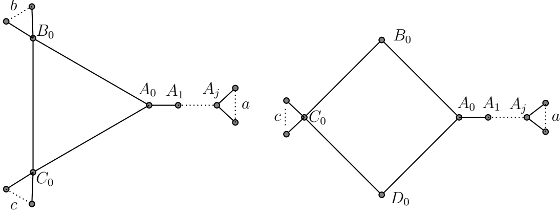
Figure 9. The graphs G_{a,b,c,j}^3 and G_{a,c,j}^4
