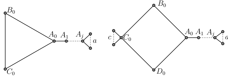
Figure 2. The graphs G_{a,j}^3 and G_{a,c,j}^4
