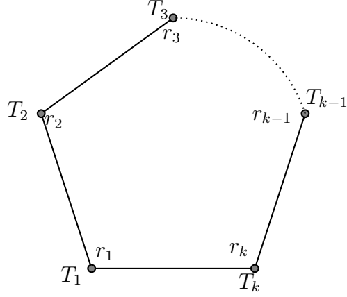
Figure 4. graph G containing C_k
