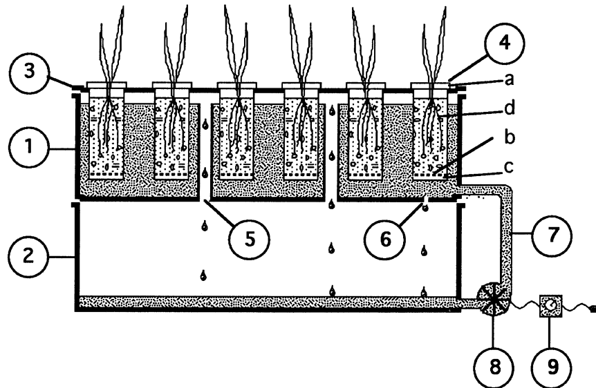
Figure 1. Diagram of the automatic immersion system (immersion phase) used for the multiplication of single cystosorus strains of Polymyxa sp. 1) Upper culture tank; 2) lower reservoir tank; 3) removable opaque lid on the upper tank with openings for insertion of culture tubes; 4) culture tube with (a) 32 mm ring (internal diameter) sealed to the tube, (b) a polyamid netting sealed to the tube with a 32 mm ring (external diameter) (c) and supporting the sand inoculum mixture (d); 5) overflow tubes sealed to the bottom of the culture tank; 6) emptying hole; 7) PVC tubing; 8) centrifugal pump; 9) timer for regulation of the alternate watering-drainage.
