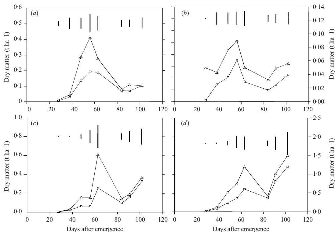
Fig. 4. Dry matter distribution ( \text{t ha}^{-1} ) in different plant components, (a) leaf, (b) leaf sheath, (c) stem and (d) total plant of millet grown with (M2, \Delta ) and without (M1, \square ) fertilizer during the 1987 growing season at the ICRISAT Sahelian Centre, Sadoré, Niger. Vertical bars represent S.E.S (D.F. = 5).
