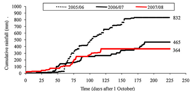
Fig. 1. Cumulative rainfall distribution at MRS during the period of experimentation.
