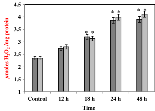
Fig. 8. Time-dependent response for H 2 O 2 production in the larvae fed on diet containing methylparathion (□) and carbofuran (■). The data represents the mean ± S.D. (n = 3). (Significantly different from control at *p < 0.01).
