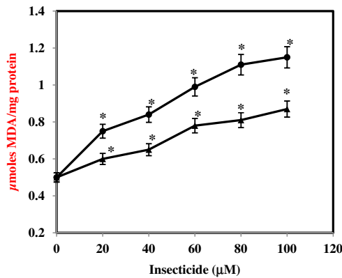
Fig. 5. Dose-dependent response for lipid peroxidation in the larvae fed on diet containing methylparathion (●) and carbofuran (▲). The data represents the Mean ± S.D. (n = 3). (Significantly different from control at *p < 0.05).
