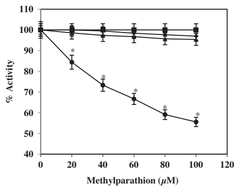
Fig. 2. Effect of methylparathion on NADH dehydrogenase (◆), succinate dehydrogenase (●), cytochrome oxidase (▲) and \text{F}_0\text{F}_1 ATPase (■) of isolated mitochondria. Enzyme activities were assessed as described in text. The data represents the Mean \pm S.D. ( n = 3 ). (Significantly different from control at *p < 0.05 ).
