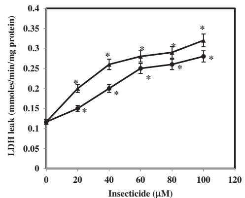
Fig. 9. Dose-dependent response for LDH leak in the larvae fed on diet containing methylparathion (●) and carbofuran (▲). The data represents the mean ± S.D. (n = 3). (Significantly different from control at *p < 0.05).
