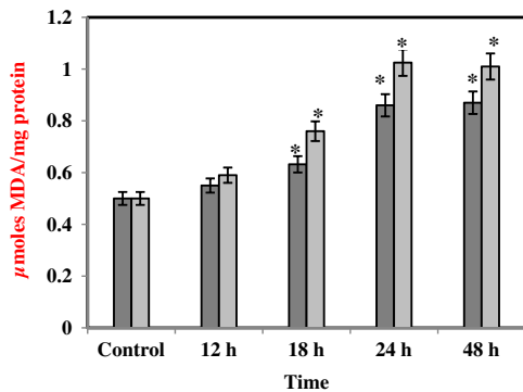
Fig. 6. Time-dependent response for lipid peroxidation in the larvae fed on diet containing methylparathion (□) and carbofuran (■). The data represents the Mean ± S.D. (n = 3). (Significantly different from control at *p < 0.05).
