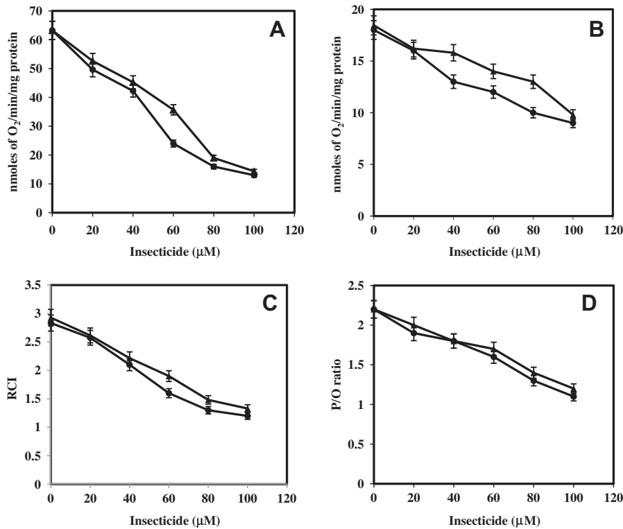
Fig. 1. Effect of methylparathion (●) and carbofuran (▲) on mitochondrial respiration when succinate was the oxidisable substrate. Conditions for oxygen uptake measurements are described in text. Insecticide was incubated for 2 min with mitochondria, prior to addition of succinate. (A) Mitochondrial oxygen uptake in the presence of ADP (state III respiration), (B) mitochondrial oxygen uptake in absence of ADP (state IV respiration), (C) RCI and (D) P/O ratio for the isolated mitochondria. The traces are the representative of three individual experiments.
