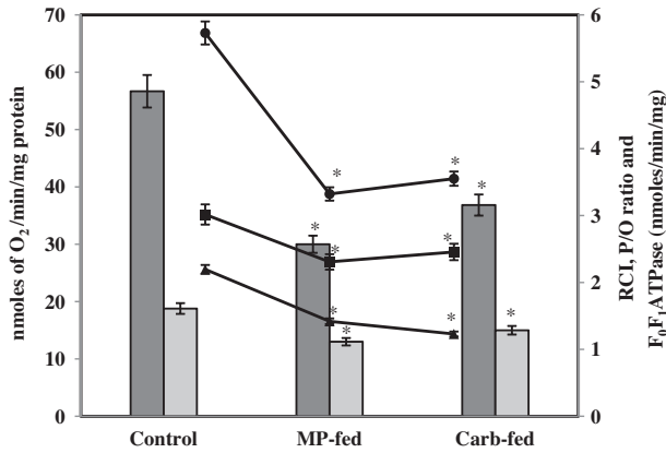
Fig. 4. In vivo effect of methylparathion and carbofuran on mitochondrial respiration for the oxidation of succinate. Oxygen consumption in presence of ADP (state III) (■), in absence of ADP (state IV) (□); RCI (■), P/O ratios (▲) and F 0 F 1 ATPase activity (●) was measured in insecticide-fed larvae as described in text. The data represents the Mean ± S.D. (n = 3). (Significantly different from control at *p < 0.05).
