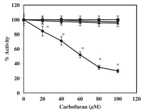
Fig. 3. Effect of carbofuran on NADH dehydrogenase (◆), succinate dehydrogenase (●), cytochrome oxidase (▲) and \text{F}_0\text{F}_1 ATPase (■) of isolated mitochondria. Enzyme activities were assessed as described in text. The data represents the Mean \pm S.D. ( n = 3 ). (Significantly different from control at *p < 0.05 ).
