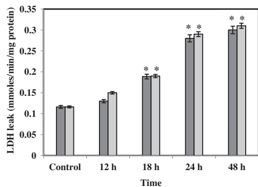
Fig. 10. Time-dependent response for LDH leak in the larvae fed on diet containing methylparathion (□) and carbofuran (■). The data represents the mean \pm S.D. ( n = 3 ). (Significantly different from control at *p < 0.05 ).
