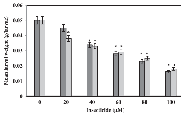
Fig. 11. Bioassay for methylparathion and carbofuran. Neonates were fed on artificial diet containing varying concentrations of methylparathion (□) and carbofuran (■). The data represents the Mean \pm S.D. ( n = 3 ) (Significantly different from control at *p < 0.05 ).
