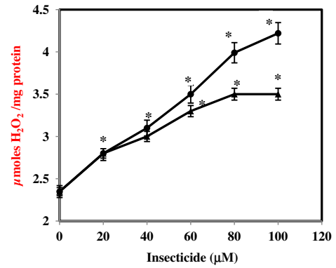
Fig. 7. Dose-dependent response for H 2 O 2 production in the larvae fed on diet containing methylparathion (●) and carbofuran (▲). The data represents the mean ± S.D. (n = 3). (Significantly different from control at *p < 0.01).
