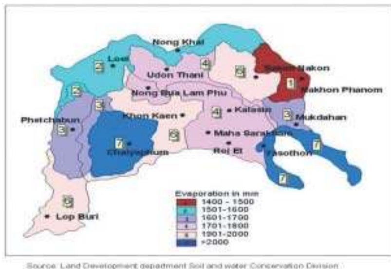
Figure 5. Evaporation map of the three watersheds: Maekhong, Chi and Pasak
