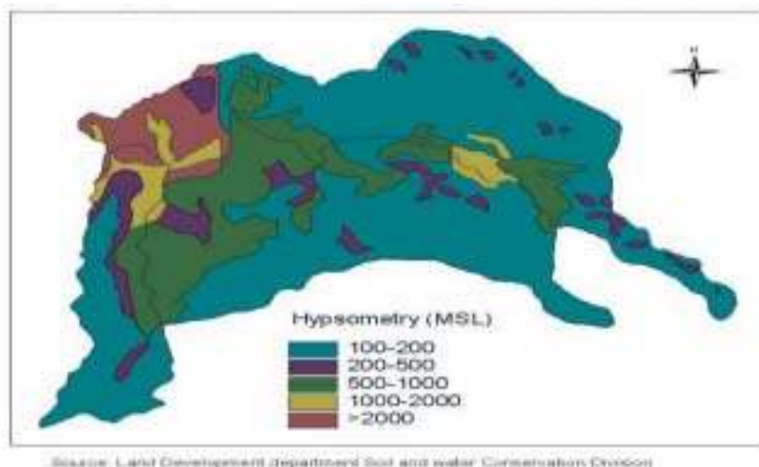
Figure 8. Hypsometry map of the three watersheds: Maekhong, Chi and Pasak.
