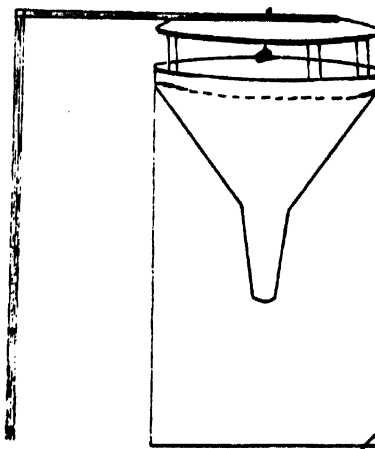
Figure 2. ICRISAT standard trap: a white plastic funnel (diameter 21 cm) with an aluminium plate rivetted above at a clearance of 5 cm. The trap is fixed with a nut and bolt and pheromone source is suspended below the plate at the centre. Moths are retained in the polythene bag wired below the funnel.
