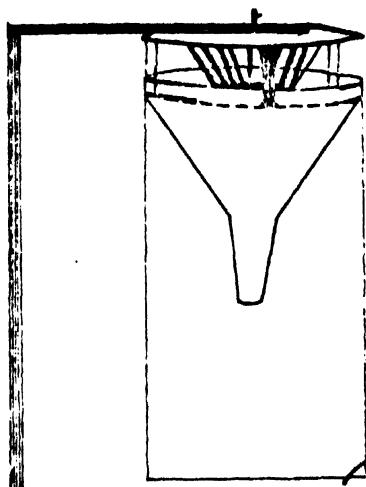
Figure 3. ICRISAT standard trap modified by inserting a perforated small yellow funnel (diameter 15 cm) around the pheromone. This funnel is secured to the aluminium plate after the placement of pheromone source below the plate.
