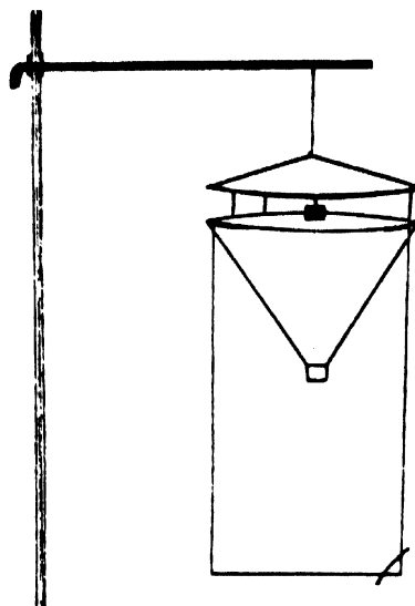
Figure 1. COPR dry funnel trap: a yellow plastic funnel (diameter 17 cm) with a hood of the same material at a clearance of 2.5 cm. The pheromone source is suspended below the hood at the centre, and moths are caught in the polythene bag wired below the funnel.
