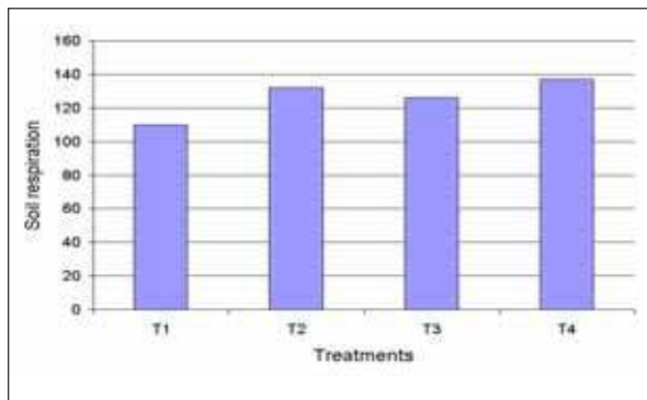
c. Soil respiration ( \text{g C g}^{-1} \text{ soil } 10\text{d}^{-1} )
