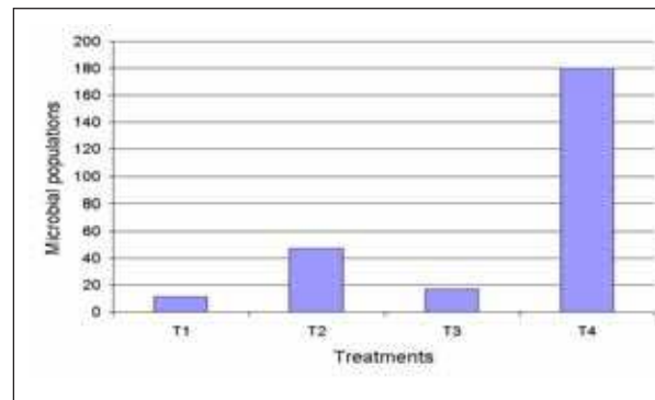
d. Mean count of microbial population ( 10^3 \text{ CFU g}^{-1} \text{ soil} )
