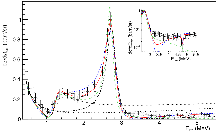
Fig. 1. (Color online.) The excitation function of the reaction ^{14}\text{O}(p, p)^{14}\text{O} measured at 180^\circ in the center of mass system. R-Matrix calculations corresponding to the ground state alone (dotted line), first excited state (thick-dot-dash line), second excited state (thin-dot-dash line) are shown. Inset: A structure clearly visible at an energy close to 4.8 MeV is assigned to the 1/2_1^- second excited state of ^{15}\text{F} (see text for details). Data are compared to the best R-Matrix fit (red line) using the properties given in Table 1. The R-Matrix calculation made with \Gamma = 737 keV for the ground state is also shown (blue dashed line) for comparison. Here, the error bars correspond to the statistical uncertainties. The calculation using the GCM-CC approach is also shown (green dotted line).
