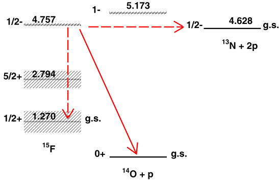
Fig. 2. (Color online.) Level scheme of ^{15}\text{F} . The possible decay channels from the J^\pi = 1/2^- resonance are: the one proton emission (red arrow), gamma transition and two proton emission (red dashed arrow). The hatched areas correspond to the width of the resonances.
