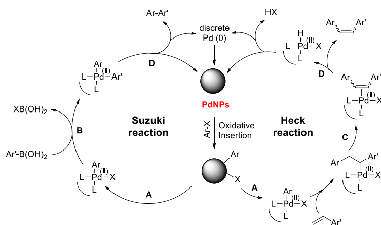
Scheme 1. Proposed mechanism of Suzuki and Heck reaction. A : chemical etching, B : transmetalation, C : \beta -hydride elimination, D : reductive elimination.
