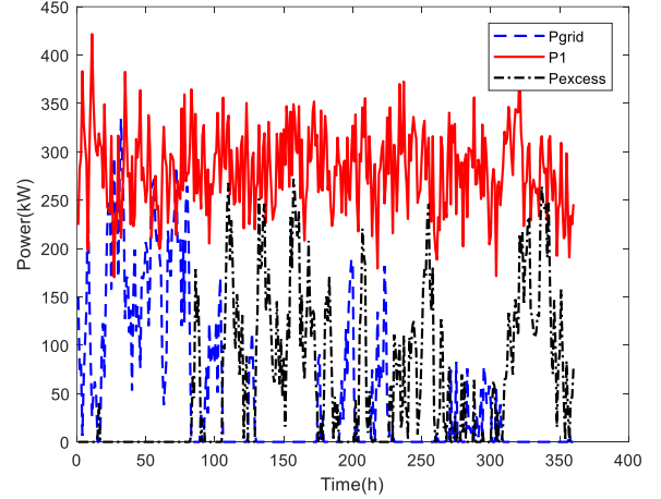
Figure 7. Power bought from grid and generated by CHP plant.
