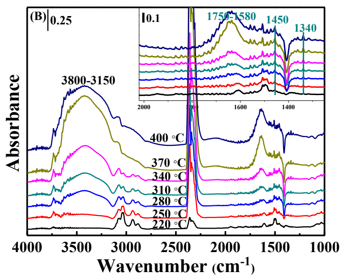
Figure 11. In situ DRIFT spectra for toluene oxidation over CCZ-SW at different temperature
