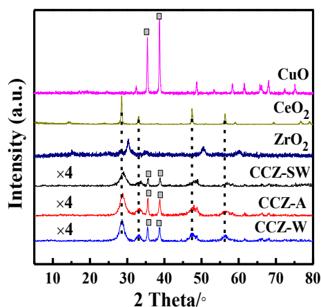
Figure 5. XRD spectra of \text{CuCe}_{0.75}\text{Zr}_{0.25}\text{O}_x catalysts
