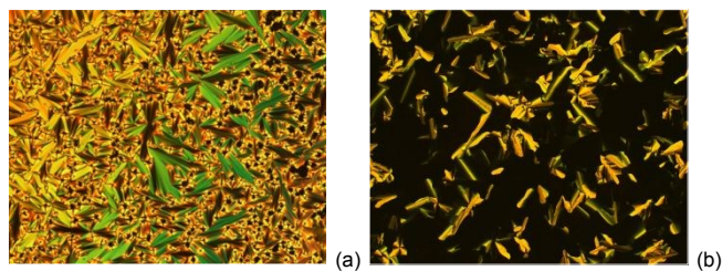
Figure 3. Optical textures taken on cooling of: (a) the SmA phase where n = 8 ; T = 162 °C; (b) the Col_h mesophase where n = 18 ; T = 163 °C.
