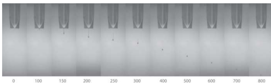
Figure 2: The time lapse images of the droplet formation of RSF from a jetting device (nozzle diameter 80 μm). The numbers below the images represent the time elapsed, in microseconds (μs), since the initiation of jetting of the silk ink droplet. Please click here to view a larger version of this figure.
