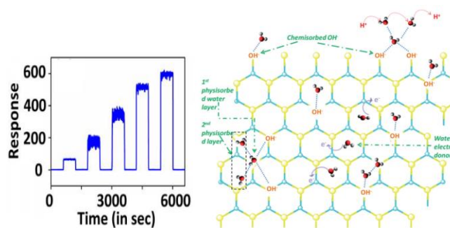
Fig. 10 (a) Response of \text{WS}_2/\text{GO} (1:3) hybrid layer for humidity [66] (b) Schematic representing proton conductivity as humidity sensing phenomenon in hybrid 2D material (reproduced from [125] with permission of Royal Society of Chemistry)
