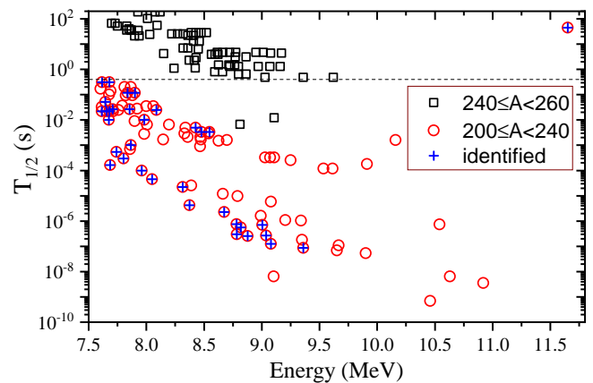
FIG. 9. Half-lives of potential candidates for two regions of nuclei with different atomic mass numbers ( 200 \leq A < 240 and 240 \leq A < 260 ) produced in the ^{48}\text{Ca} + ^{249}\text{Bk}/^{249}\text{Cf} reactions are shown by open symbols as function of their \alpha -particle energies. Only those \alpha -decay branches with absolute intensities and \alpha -particle energies exceeding 10% and 7.6 MeV, respectively, are compiled. Isotopes identified in the analysis of the present data are marked by plus-signs. A time level of 0.4 s at which most of the data can be separated into two groups is indicated by the dashed line.
