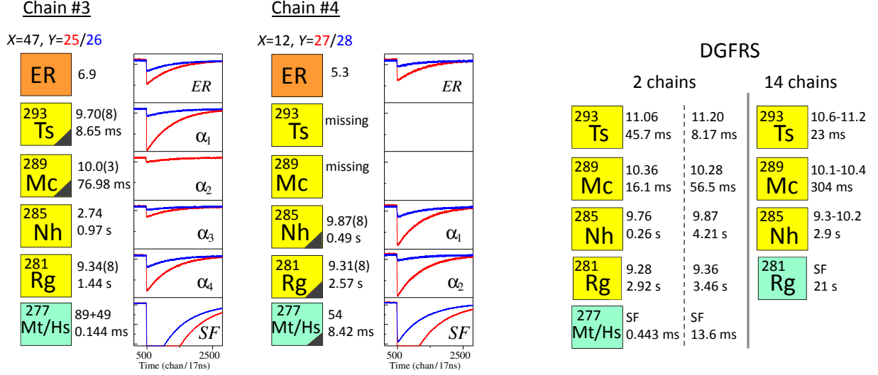
FIG. 7. Suggested decay sequence of two short \alpha -decay chains observed during the 254 MeV-run (chain #3) and 258 MeV-run (chain #4). Summaries of the sixteen short decay chains observed at DGFRS and attributed to the decay of ^{293}\text{Ts} [20–23] are also shown for comparative discussion. Energies and correlation times of all individual members are given for two DGFRS chains that end by fission of either ^{277}\text{Mt} or ^{277}\text{Hs} . For each member of the “14 chains”, an average half-life was calculated from those data, where the correlation time was measured relative to the mother nucleus. Isotopic assignments of chains #3 and #4 are made based on the DGFRS findings. In the case of chain #4 only one of several possible scenarios is given. Boxes with black triangles indicate events observed during beam-off periods. The measured fission fragment energies are from stop+box detectors. The corresponding traces of all members of the chains are shown on the right side of the chains. For more details, see text.
