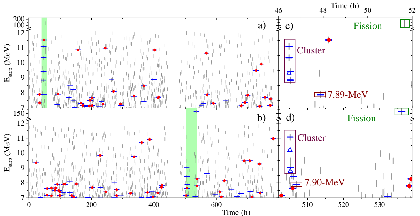
FIG. 5. Stop detector energies of anti-MWPC (vertical lines) and beam-off (horizontal lines) events in the pixels X/Y=103/41 (a) and 111/19 (b) are shown as function of time, start from the beginning of the experiment. In the left panels, the time scale covering the entire experiment is shown. Shaded regions mark time windows where the chains #1 and #2 and fissions were detected. An expanded view of the time around these shaded regions is shown in the right panels (c,d). Identified beam-off \alpha -like events with energies 7-12 MeV are marked by squares. In right panels, the \alpha members of cluster-events reconstructed from stop and box detectors are shown by triangles. For details, see text.
