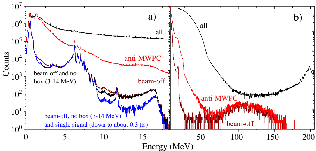
FIG. 3. Low a) and b) high energies spectra measured during the 270 MeV-run. All, anti-MWPC, and beam-off events are shown. In a) the spectrum of beam-off events detected solely with the stop detector or no coincidence box detector signal within energies 3-14 MeV is shown. The spectrum of these events with the additional requirement of having only single-signal traces (digital part of CANDI) is also shown. The algorithm for testing a presence of multi-signal traces has a time limit down to 0.3 \mu\text{s} in between signals.
