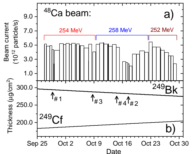
FIG. 1. a) Average beam currents for each run (254 MeV, 258 MeV and 252 MeV). b) Evolution of isotopic thicknesses of ^{249}\text{Bk} and ^{249}\text{Cf} with average total thickness of 0.48(5) \text{ mg}/\text{cm}^2 during the irradiations by ^{48}\text{Ca} beam with energies E_{\text{lab}} = 254.0, 258.0 and 252.1 MeV. Arrows indicate the dates when the long (#1 and #2) and short (#3 and #4) chains were detected.
