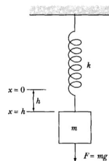
Fig. 1. Illustration of the set-up for the simple harmonic oscillator. Image taken from Thorton and Marion (2004)
