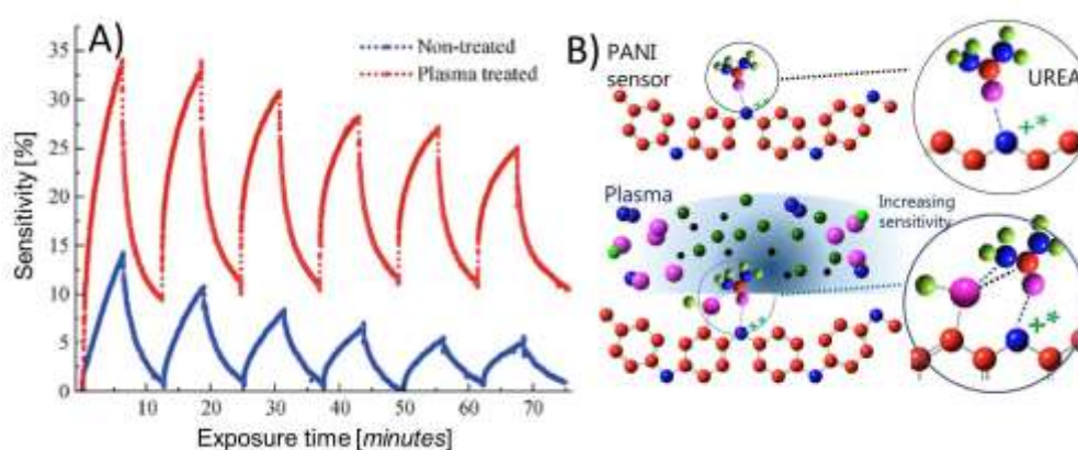
Figure 9. (a) Response of pristine and atmospheric pressure plasma treated PANI towards 15 ppm of urea and (b) sensing mechanism in pristine and plasma modified PANI. (Reproduced with permission from. [65] Courtesy and copyright: Higher Education Press and Springer-Verlag Berlin Heidelberg 2016.
