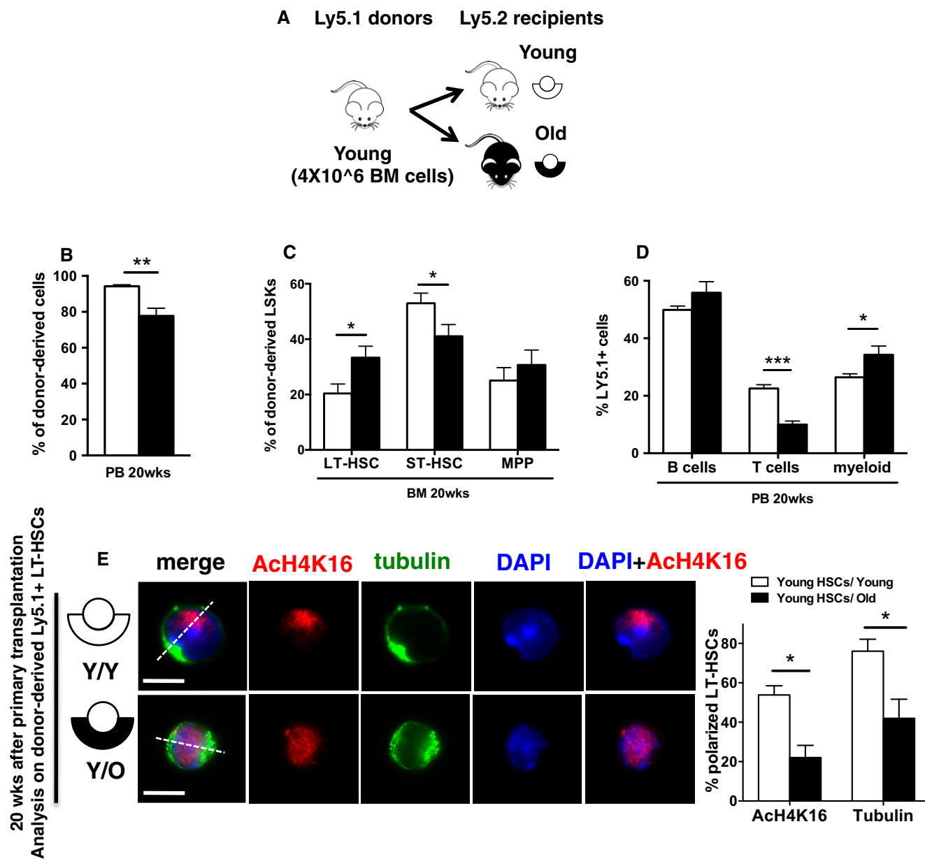
Figure 1. Transplantation of young BM cells into an aged microenvironment causes HSC expansion and myeloid development.
