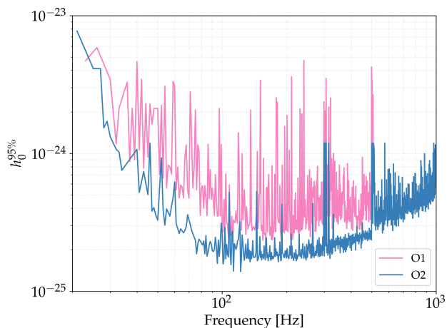
FIG. 6. Comparison of O1 and O2 95% upper limits on the strain amplitude for the FrequencyHough pipeline. The O2 search covered the range between 20 Hz and 1000 Hz, while the O1 search arrived up to 475 Hz. They have been obtained adding simulated signals to the real data, covering the same parameter space as in the actual search.
