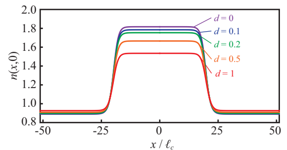
FIG. 6. Asymptotic stationary concentration distributions of passive particles for different equilibrium diffusion coefficients inside the raft. The ratios d = D_0/D_\infty are indicated next to each curve. Other parameters are R = 20\ell_c , \delta = 2\ell_c , and \xi/D_\infty = 1 .
