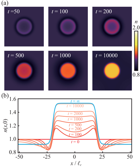
FIG. 3. Accumulation of passive particles by a raft occupied with active proteins. (a) Consequent snapshots of the concentration distribution and (b) radial profiles at different time moments are displayed. The final profile ( t = \infty ) is determined using the analytical solution (19). The parameters are R = 20\ell_c , \delta = 2\ell_c , and \xi/D_T = 1 . The corresponding movie is available in the Supplemental Material [21].
