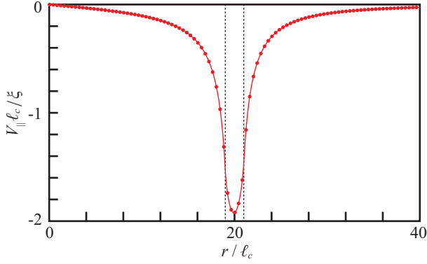
FIG. 7. Profiles of the radial component of the velocity, V_{\parallel} , obtained by the numerical integration (solid circles) and analytical calculation (solid curves) in the case with a circular raft of a radius R , in which the concentration of active proteins is c_0 . We set R/\ell_c = 20 , just as in Fig. 1. The parameter \delta in Eq. (15) is set as \delta = 0 .
