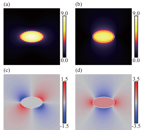
FIG. 2. Diffusion enhancement for an elliptic raft with the semiaxes 20\ell_c and 10\ell_c and the sharp boundary. The diffusion enhancement components (a) D_{11}^A/\xi , (b) D_{22}^A/\xi , and (c) D_{12}^A/\xi are displayed. (d) The diffusion anisotropy ( D_{11}^A - D_{22}^A )/ \xi is additionally shown.
