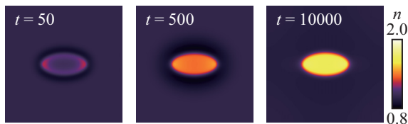
FIG. 4. Accumulation of passive particles by an elliptic raft. Consequent snapshots of the concentration distribution at three time moments are displayed. The major and minor semiaxes of the ellipse are 20\ell_c and 10\ell_c . Other parameters are \delta = 2\ell_c and \xi/D_T = 1 . The corresponding movie is available in the Supplemental Material [21].
