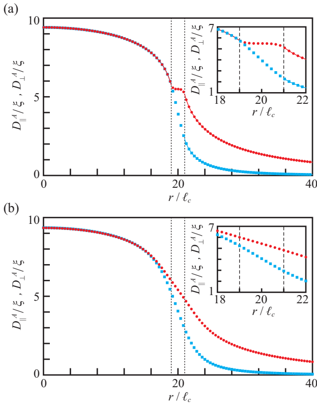
FIG. 1. Diffusion enhancement by a circular raft of radius R = 20\ell_c with the boundary width (a) \delta = 0 and (b) \delta = 2\ell_c . The profiles of diffusion enhancement in the radial, D_{\parallel}^A/\xi (red, dark gray), and in the transverse, D_{\perp}^A/\xi (cyan, light gray), directions as a function of the distance from the raft center are shown.
