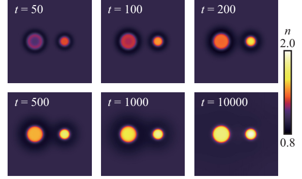
FIG. 5. Accumulation of passive particles by two rafts of different sizes. Consequent snapshots of the concentration distribution are displayed. The parameters are R_1 = 10\ell_c , R_2 = 6\ell_c , \delta = 2\ell_c , and \xi/D_T = 1 . The corresponding movie is available in the Supplemental Material [21].
