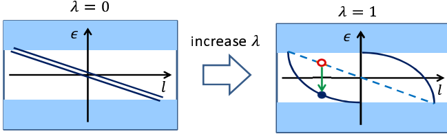
FIG. 2. Schematic picture of the spectrum of a chiral d -wave superfluid for the smooth confinement potential (left) and sharp confinement potential (right). \lambda characterizes the potential shape. Some eigenvalues changes the sign as indicated by the green arrow.
