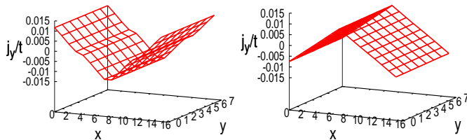
FIG. 7. Mass current density along the y -direction for \theta = 0 (left) and \theta = \pi (right). The parameters are V_0 = -t, \mu = -2.2t . The chirality of \Delta^0 is positive for 0 \leq x < L_x = 8 , while it is negative for L_x \leq x < 2L_x = 16 .
