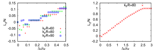
FIG. 8. OAM for the Hamiltonian Eq. (16). \Delta_0 dependence for different system sizes (left panel), and global \Delta_0 dependence for the fixed system size k_F R = 80 (right panel).
