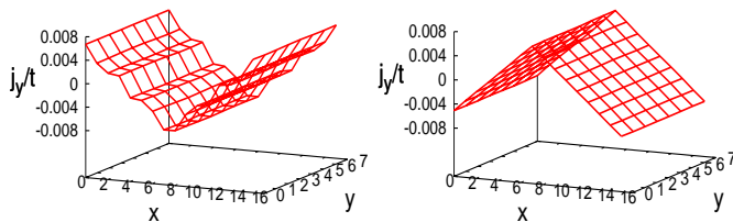
FIG. 6. Mass current density along the y -direction for \theta = 0 (left) and \theta = \pi (right). The parameters are V_0 = -0.1t, \mu = -t . The chirality of \Delta^0 is positive for 0 \leq x < L_x = 8 , while it is negative for L_x \leq x < 2L_x = 16 .
