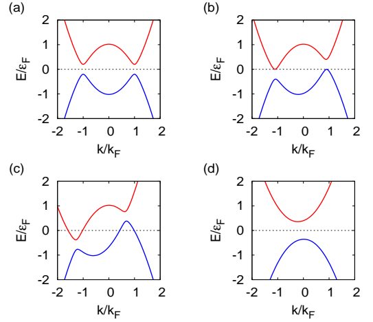
FIG. 4. Dispersions in the BCS states in one-dimension at \mu = \varepsilon_F , \Delta_0 = 0.2\varepsilon_F for (a) v_s = 0 , (b) v_s = v_L , and (c) v_s = 3v_L , where v_s = |\mathbf{q}|/2m_0 and v_L = \Delta_0/k_F . (d) Dispersion in the BEC state at \mu = -0.3\varepsilon_F , \Delta_0 = 0.2\varepsilon_F , v_s = v_L . Red curve is E_{k1} and blue curve is E_{k2} .
