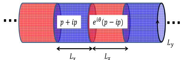
FIG. 5. Infinite length cylinder with the circumference L_y . Each domain size is L_x \times L_y .
