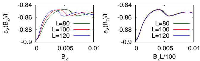
FIG. 1. (Left panel) The ground state energy density at \Delta_0 = 0.6t for different system sizes. The dimensionless magnetic flux density is B_z = \phi/2\pi where \phi is the flux per plaquette of the square lattice. (Right panel) The ground state energy density in the scaling plot.
