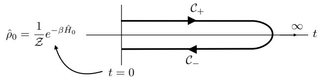
Figure 1. Closed semi-infinite time contour employed in the path-integral formulation of the quench problem studied in this work. At the initial time t = 0 our system is in a thermal state of the non-interacting noiseless Hamiltonian H_0 given in (8).
