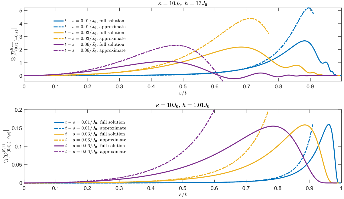
Figure 5. (Color online). Behavior of the correlation of the longitudinal magnetization as a function of the ratio of the two times, both away (upper panel) and close to (lower panel) the critical point. Different colors correspond to different values of the time difference. The dashed lines indicate the asymptotic solution at small times from (2) of the two-time correlation function.
