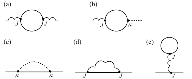
Figure 2. Diagrammatic expression of the Gaussian action for the magnetization field \mathcal{M} (wiggly lines), leading to the Langevin equation (18). The dimensionless noise field \eta/\kappa is indicated by a dashed line while the Schwinger boson by a solid line. The magnetization couples to the bosons with coupling constant J_{ij} while the dimensionless noise field with coupling constant \kappa . The non-equilibrium Green's functions are computed on the semi-infinite real-time closed contour of Fig. 1. Contour indices as well as bosonic spin indices are suppressed. The Gaussian action is defined by diagrams (a) plus (b), whereby the bosonic loops are computed using the Green's functions dressed by the self-energy insertions (c), (d), and (e).
