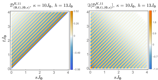
Figure 3. (Color online). Response and correlation function of the longitudinal magnetization (see (25) and (26)) far away from the critical point.
