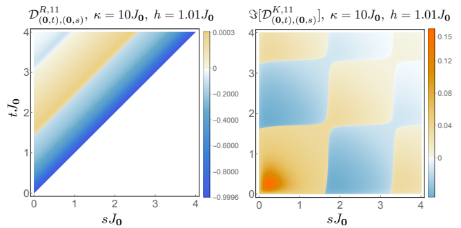
Figure 4. (Color online). Response and correlation functions of the longitudinal magnetization (see (25) and (26)) close to the critical point.
