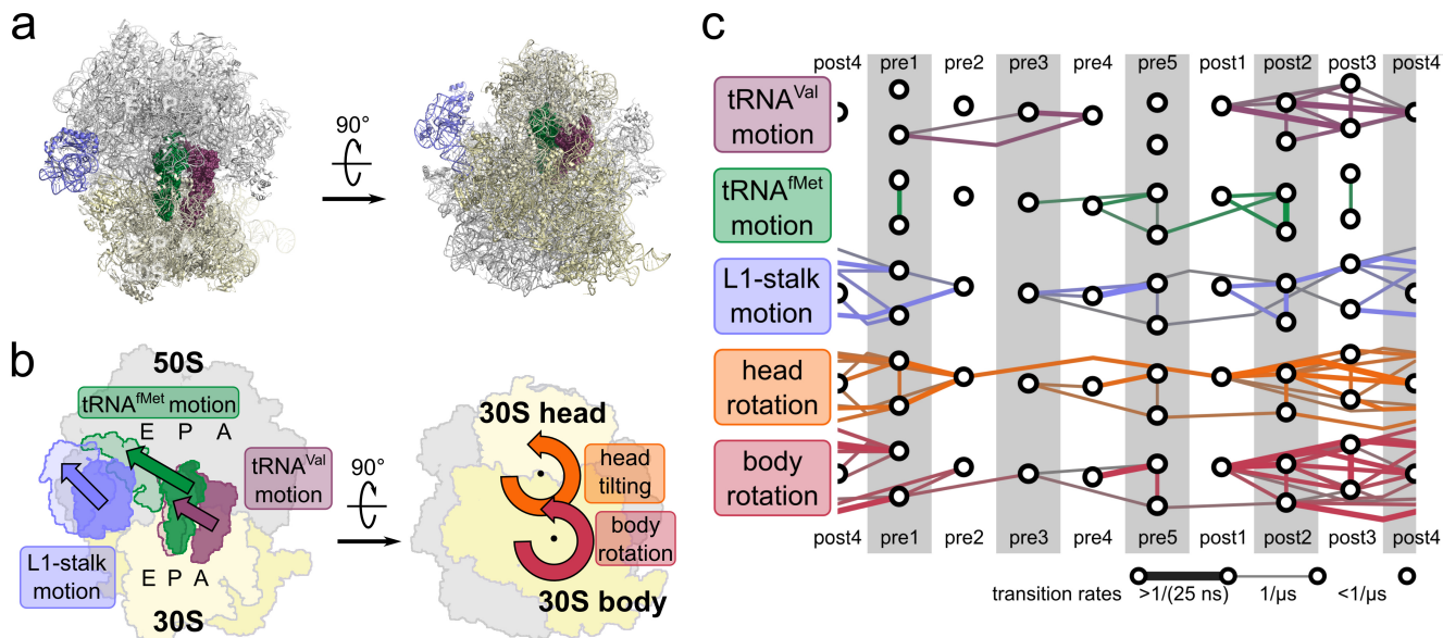
Figure 3: (a) Pre-translocation structure of the ribosome with tRNAs in A and P sites (purple, green). (b) Motions accompanying tRNA translocation. (c) Transition rates for different motions between different states estimated from the simulations. Figure adapted from Ref. 14.
