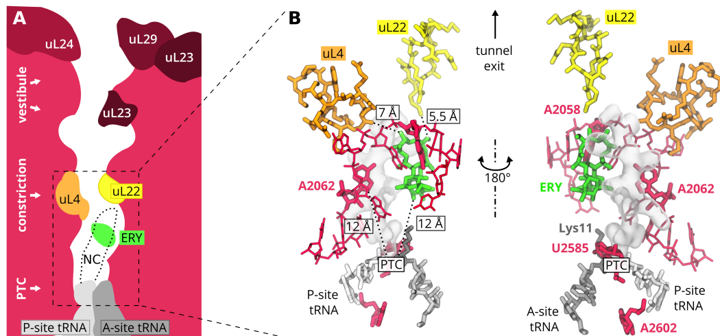
Figure 2: A: Scheme of the ribosome exit tunnel with several proteins highlighted. NC, nascent chain; ERY, erythromycin; PTC, peptidyl transferase center. B: Context of the erythromycin (ERY, in green) binding; figure based on PDB: 5JTE. 6 Several large subunit nucleotides are highlighted in bold red. Two proteins uL4 and uL22 form a constriction site. The nascent peptide is shown as transparent surface.
