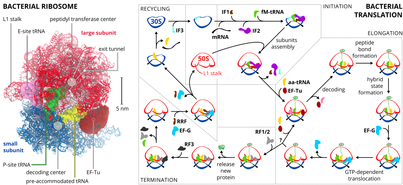
Figure 1: Structure of the bacterial ribosome in complex with EF-Tu (PDB 5AFI 3 ). Scheme of the bacterial translation cycle as reviewed in Ref. 4. 30S: small subunit; 50S: large subunit; IF1, IF2, IF3: initiation factors; fM-tRNA: N-formylmethionine tRNA; aa-tRNA: aminoacyl tRNA; EF-Tu, EF-G: elongation factors; RF1, RF2, RF3: release factors; RRF: ribosome recycling factor; green trace: nascent protein. The question mark stands for a stop codon recognition.
