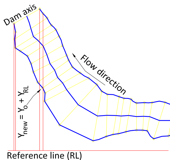
Figure S1. Transformation of Tarbela Reservoir Sedimentation Survey's local coordinates to global coordinates (Cartesian coordinates system) using AutoCAD Civil 3D 2018
