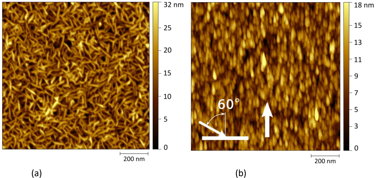
Figure 3: AFM images of the target before (a) and after (b) ion irradiation with a total Ar fluence of 8 \times 10^{21} \text{ m}^{-2} show a significant change of the surface structure. An initial nano-scale structure on an unirradiated sample transforms into a structure clearly aligned in the direction of irradiation (indicated by the white arrow) [18].
