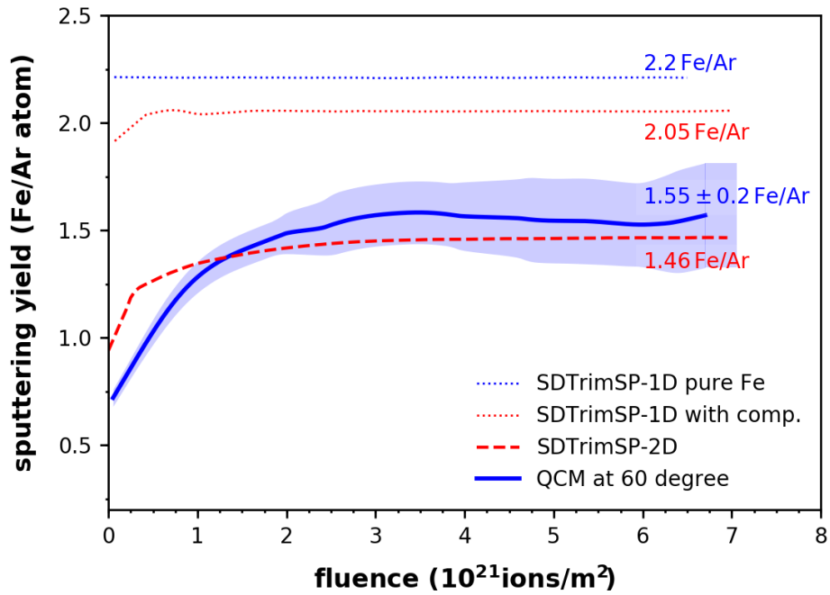
Figure 5: Measured sputtering yield for 500 eV Ar ions bombarding an iron film under an angle of incidence of 60 degree, as a function of the Ar ion fluence (thick blue line). The increase of the sputtering yield at low fluences corresponds to the sputtering of the oxide layer. The dotted and dashed lines represent numerical simulations with SDTrimSP-1D and 2D. Taking into account the actual elemental composition of the target improves the 1D-simulation (red dotted line) somewhat. By including the surface morphology in a SDTrimSP-2D simulation (thick red dashed line) the agreement with experimental results is substantially improved.
