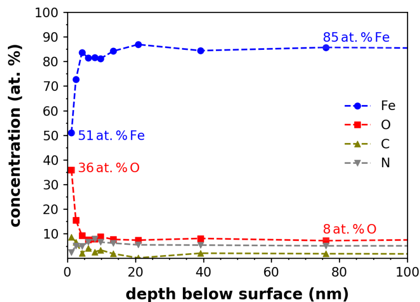
Figure 2: The XPS analysis of the Fe-film as function of depth shows a significant oxide layer on top of the sample.
