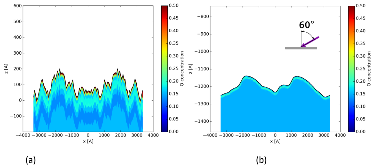
Figure 4: (a) The model surface used as input for the SDTrimSP-2D simulations. The color represents the O concentration in the respective depth. The x-axis represent the lateral position along the surface and the z-axis the depth relative to the unirradiated surface. The surface was defined to have the same distribution of local impact angles and RMS value as derived from the AFM image in figure 3a. (b) After irradiation with 500 eV Ar ions up to a total Ar fluence of 8 \times 10^{21} \text{ m}^{-2} impinging under a nominal angle of incidence of 60 degree from the right, the simulations show a smoothing of the surface consistent with the experimental data presented in figure 3. Additionally oxygen depletion at the surface occurs.
