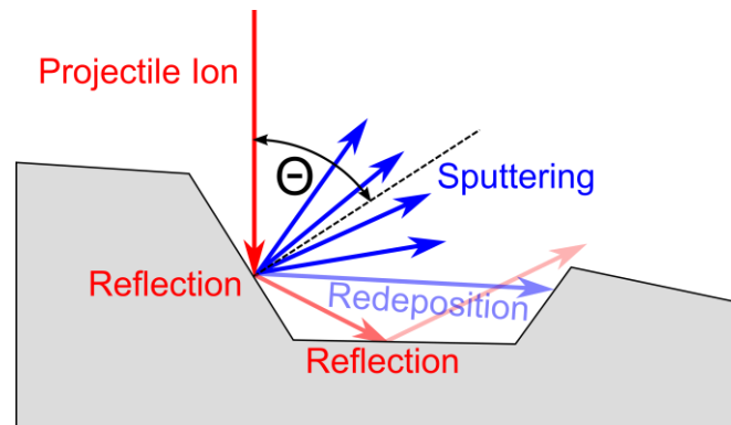
Figure 1: Sputtering of a rough surface. A projectile ion, which is represented by the red arrow, hits a surface under nominal normal incidence. However due to the surface structure the local angle of incidence \theta differs from 0 degree and thus affects the sputtering yield. Some of the sputtered atoms cannot escape the surface and get redeposited, while multiple reflections of the projectile ion may lead to further erosion of the surface (after [10]).
