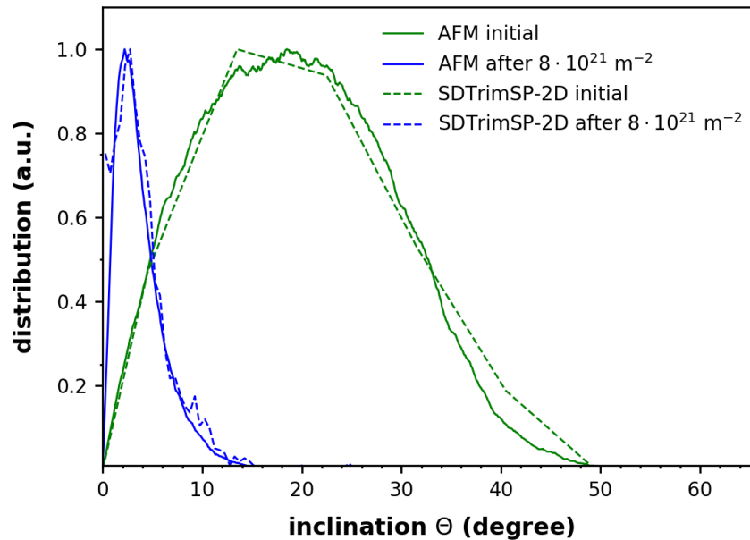
Figure 7: The distributions of local impact angle \theta (i.e. the angles between the direction of the incident projectile and the local surface normal) as derived from the AFM images in figure 4, show a shift towards lower angles and a decrease in width after ion-beam irradiation. The dashed lines show the results of numerical simulations with SDTrimSP-2D.
