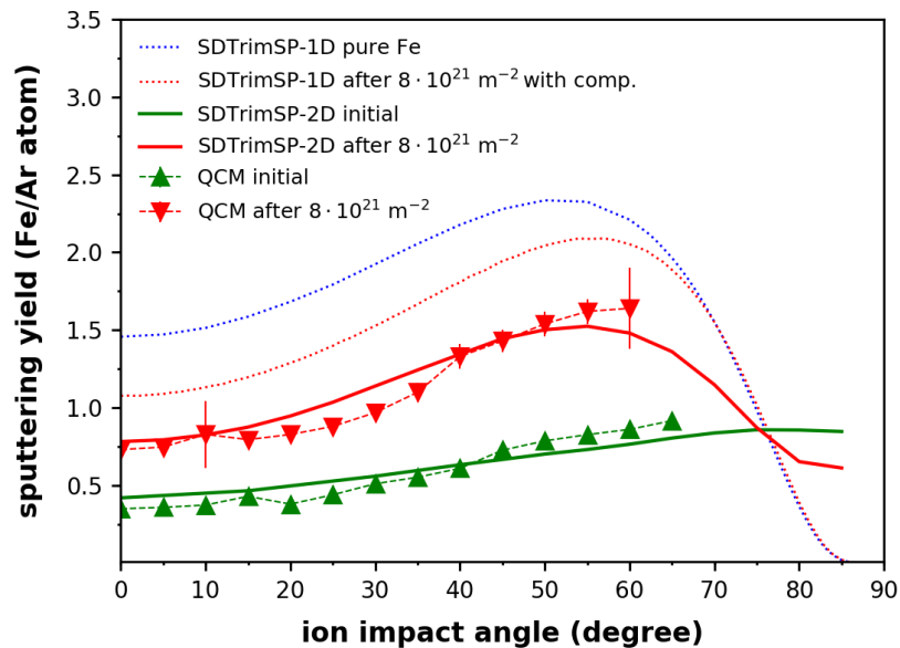
Figure 6: The green triangles give the measured Fe sputtering yield as a function of nominal impact angle for the initial target surface. A simulation with SDTrimSP-2D (green curve) which includes both the measured surface roughness (from AFM) and elemental composition (from XPS) fits the experimental data better than a static 1D simulation with SDTrimSP assuming a flat surface and a pure Fe target (blue dotted curve). The agreement remains excellent when comparing the experimental data for the Fe film (red inverted triangles) irradiated with a total Ar fluence of 8 \times 10^{21} \text{ m}^{-2} with a fully dynamic SDTrimSP-2D simulation starting from the initial situation given in figure 4a. The SDTrimSP-1D simulation, which includes also the elemental depth composition with a flat surface (red dotted line) show a good qualitative agreement, but the absolute values are too high.
